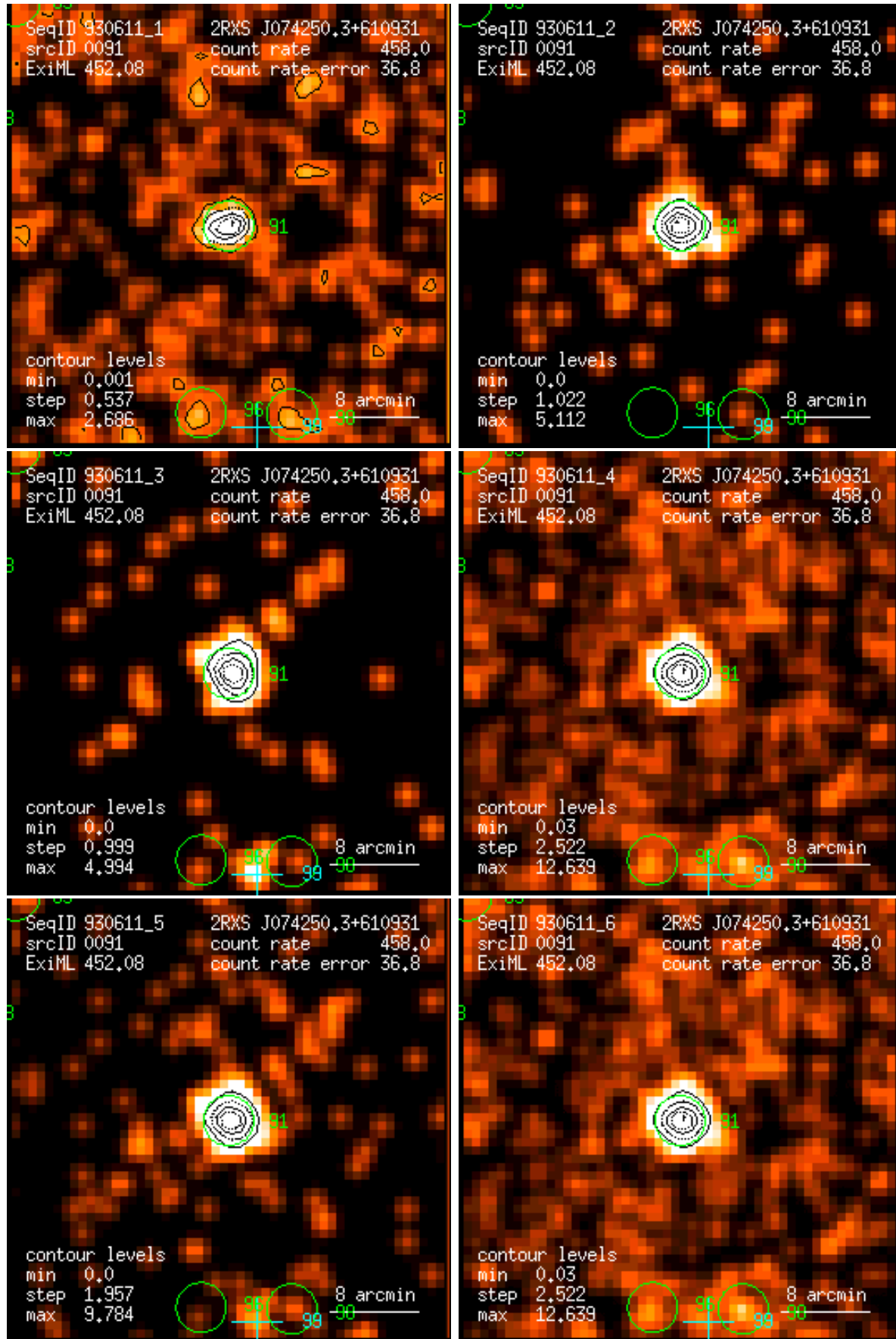
Figure 91: RASS 930611: detection 0091: band rate images, Gaussian filter: (1) PSPC channels 11 – 41, (2) 52 – 90, (3) 91 – 201, (4) 11 – 235, (5) 52 – 201, (6) 11 – 201. Broad band rates in counts/ks. Band rate contour levels in counts/ks/arcmin 2 .
