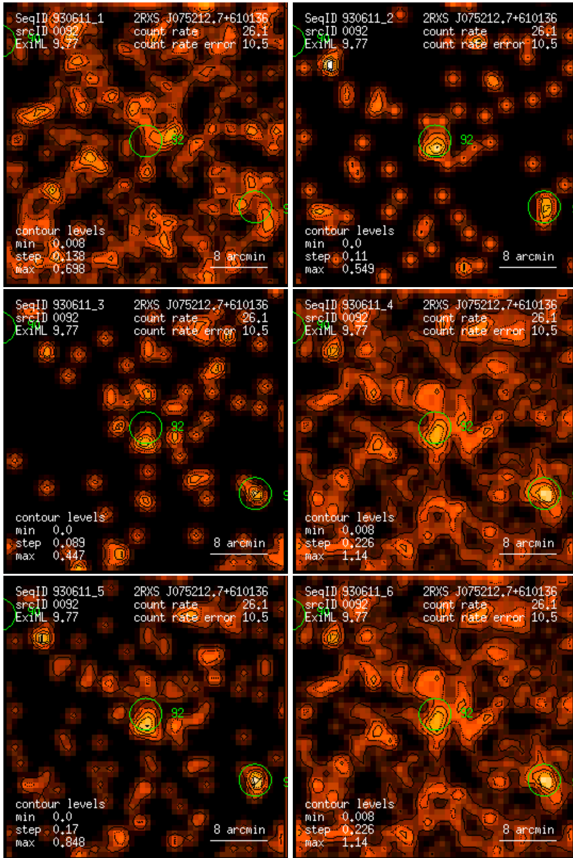
Figure 92: RASS 930611: detection 0092: band rate images, Gaussian filter: (1) PSPC channels 11 – 41, (2) 52 – 90, (3) 91 – 201, (4) 11 – 235, (5) 52 – 201, (6) 11 – 201. Broad band rates in counts/ks. Band rate contour levels in counts/ks/arcmin 2 .
