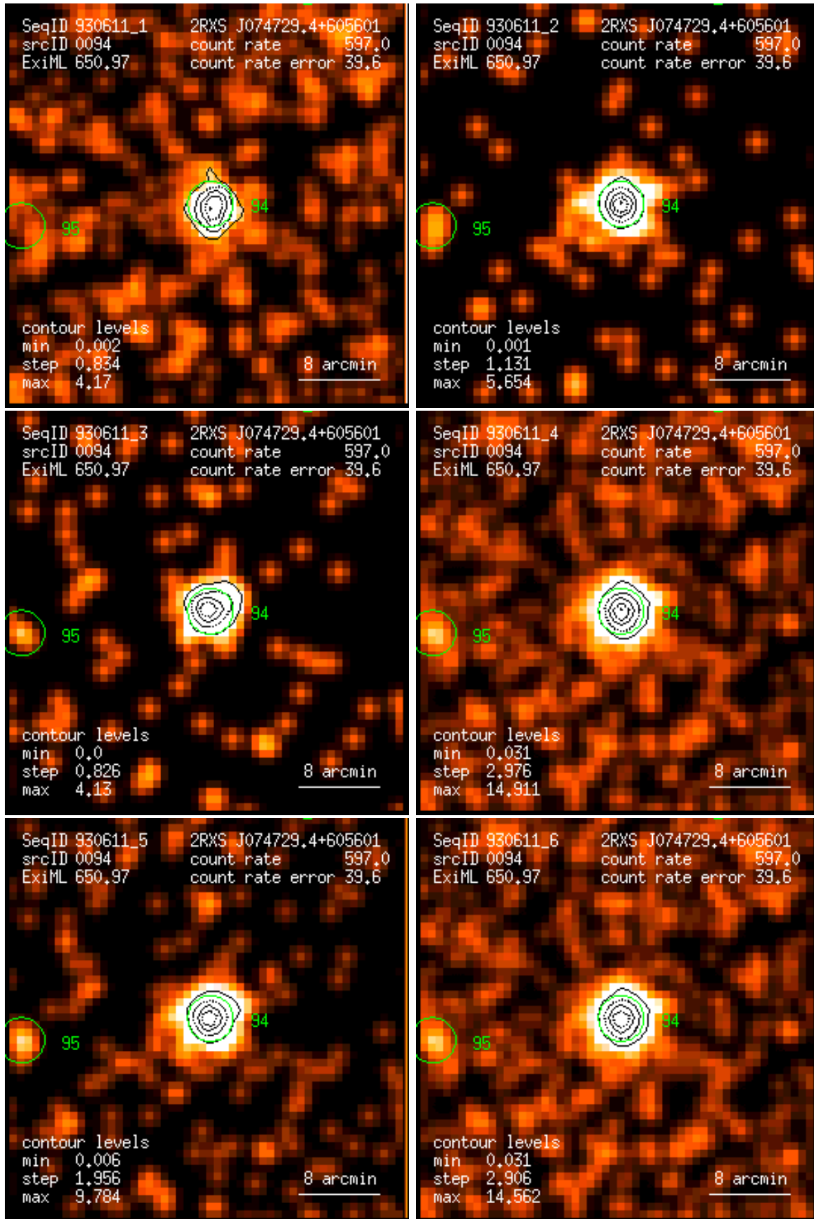
Figure 94: RASS 930611: detection 0094: band rate images, Gaussian filter: (1) PSPC channels 11 – 41, (2) 52 – 90, (3) 91 – 201, (4) 11 – 235, (5) 52 – 201, (6) 11 – 201. Broad band rates in counts/ks. Band rate contour levels in counts/ks/arcmin 2 .
