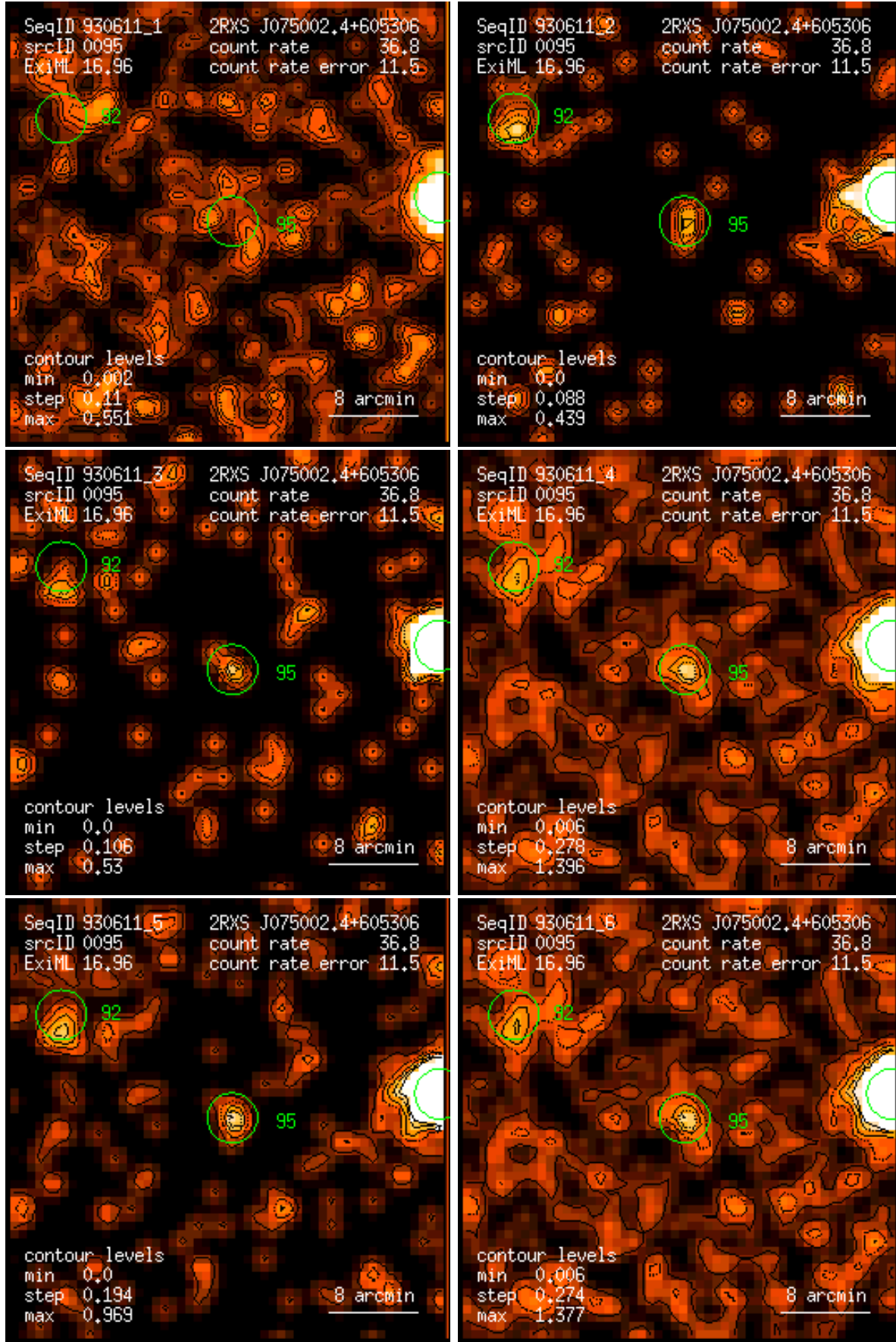
Figure 95: RASS 930611: detection 0095: band rate images, Gaussian filter: (1) PSPC channels 11 – 41, (2) 52 – 90, (3) 91 – 201, (4) 11 – 235, (5) 52 – 201, (6) 11 – 201. Broad band rates in counts/ks. Band rate contour levels in counts/ks/arcmin 2 .
