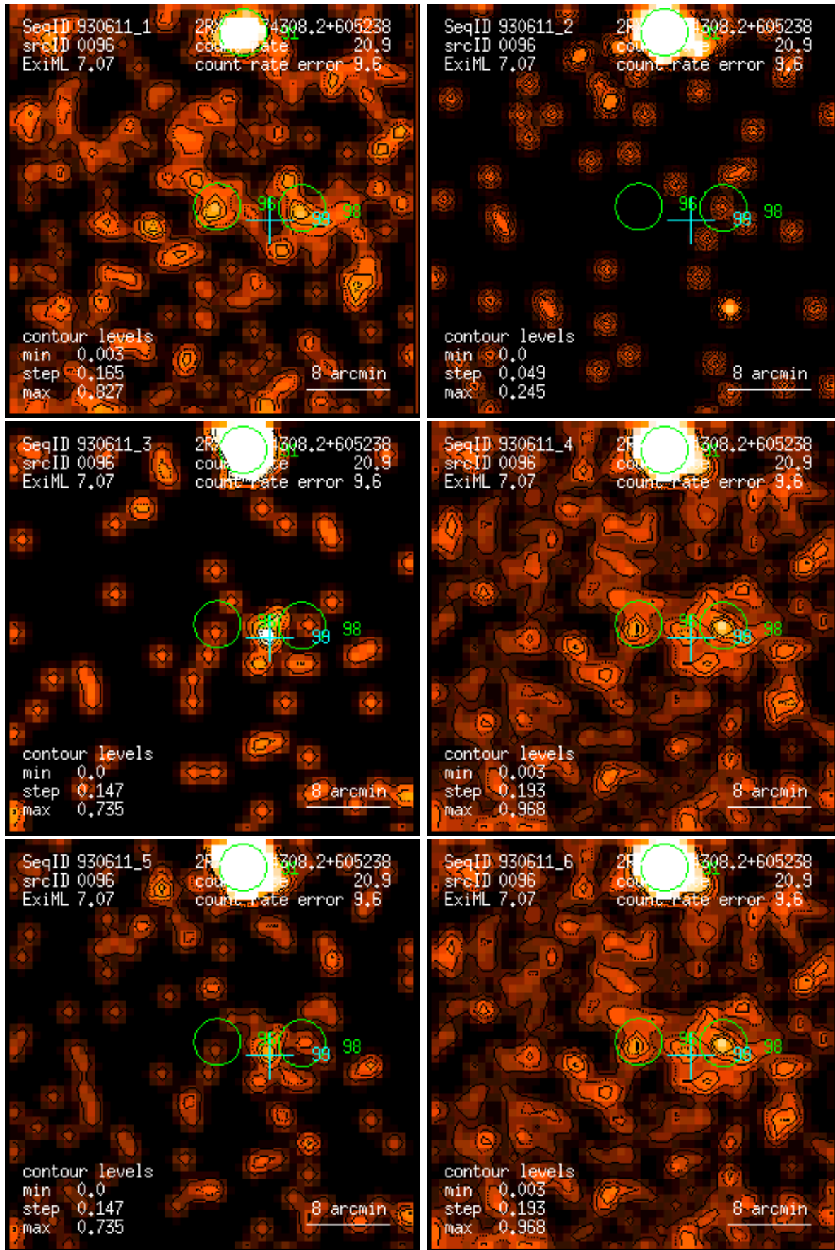
Figure 96: RASS 930611: detection 0096: band rate images, Gaussian filter: (1) PSPC channels 11 – 41, (2) 52 – 90, (3) 91 – 201, (4) 11 – 235, (5) 52 – 201, (6) 11 – 201. Broad band rates in counts/ks. Band rate contour levels in counts/ks/arcmin 2 .
