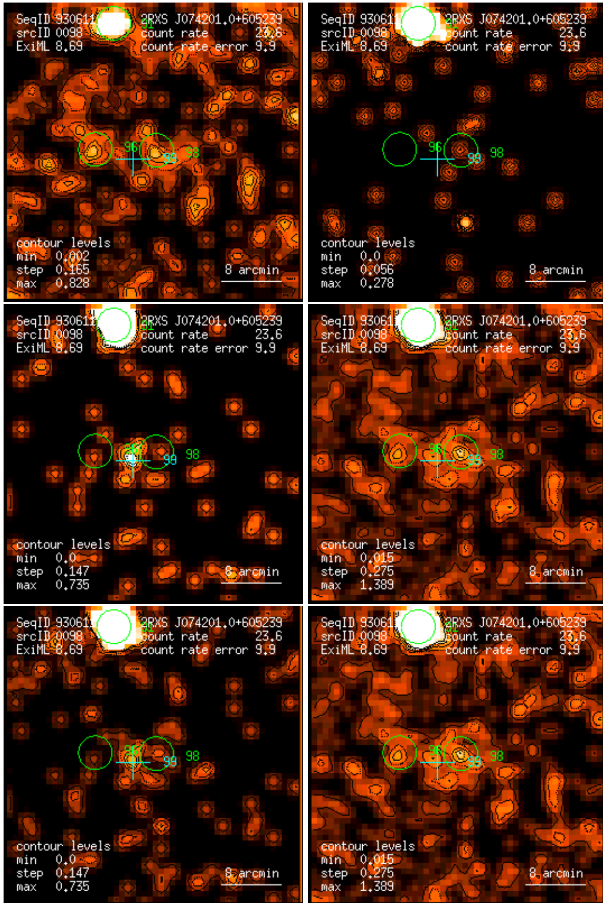
Figure 98: RASS 930611: detection 0098: band rate images, Gaussian filter: (1) PSPC channels 11 – 41, (2) 52 – 90, (3) 91 – 201, (4) 11 – 235, (5) 52 – 201, (6) 11 – 201. Broad band rates in counts/ks. Band rate contour levels in counts/ks/arcmin 2 .
