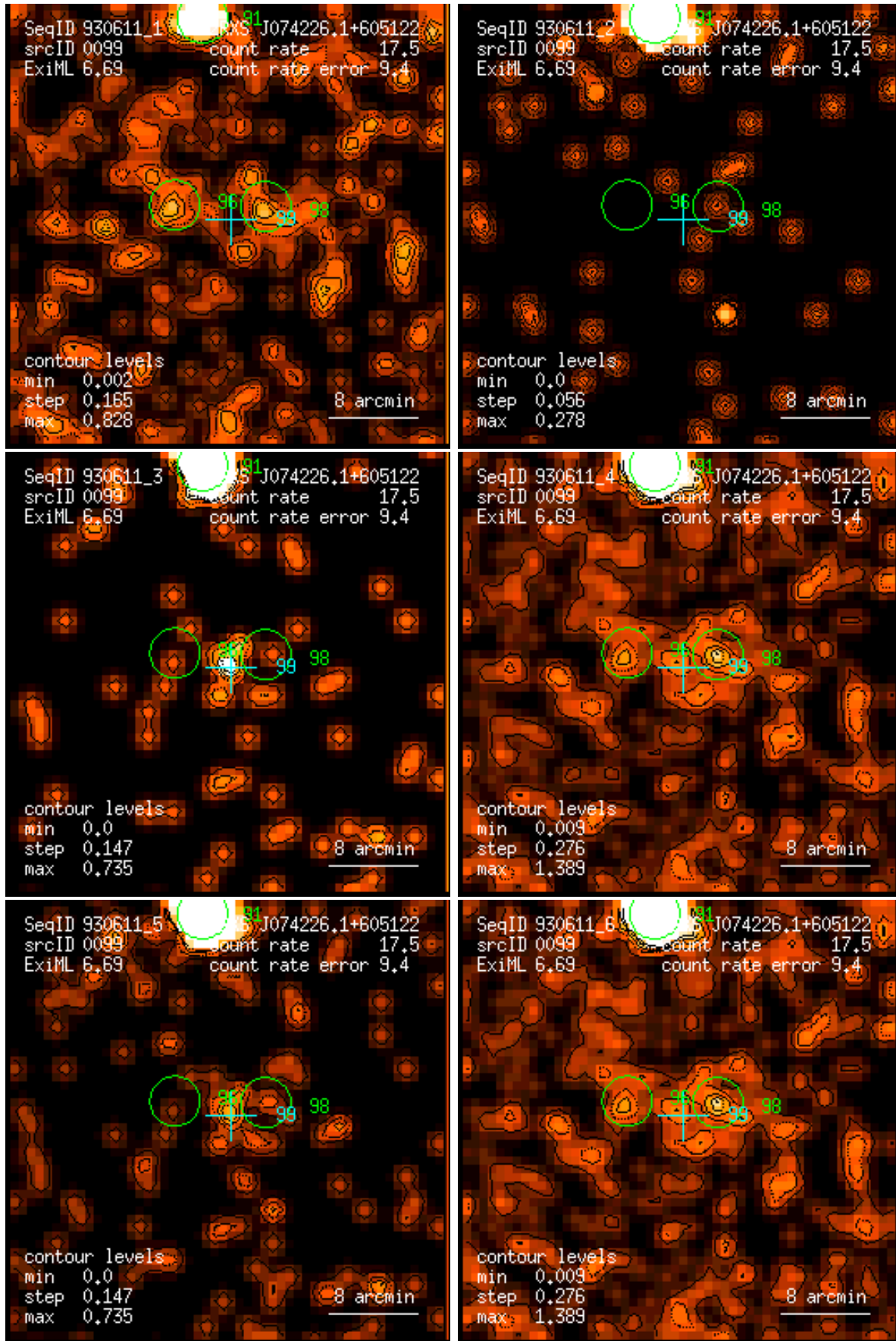
Figure 99: RASS 930611: detection 0099: band rate images, Gaussian filter: (1) PSPC channels 11 – 41, (2) 52 – 90, (3) 91 – 201, (4) 11 – 235, (5) 52 – 201, (6) 11 – 201. Broad band rates in counts/ks. Band rate contour levels in counts/ks/arcmin 2 .
