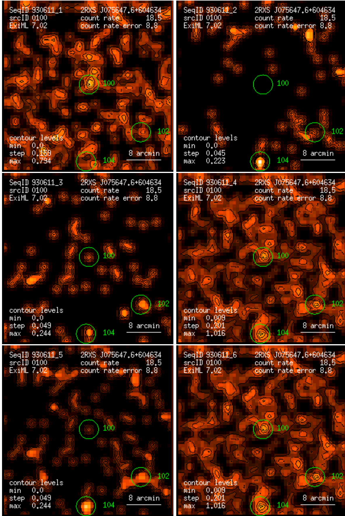
Figure 100: RASS 930611: detection 0100: band rate images, Gaussian filter: (1) PSPC channels 11 – 41, (2) 52 – 90, (3) 91 – 201, (4) 11 – 235, (5) 52 – 201, (6) 11 – 201. Broad band rates in counts/ks. Band rate contour levels in counts/ks/arcmin 2 .
