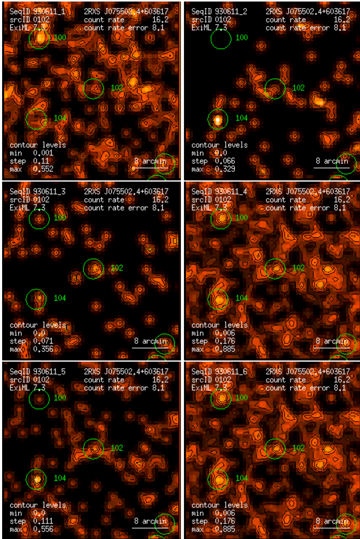
Figure 102: RASS 930611: detection 0102: band rate images, Gaussian filter: (1) PSPC channels 11 – 41, (2) 52 – 90, (3) 91 – 201, (4) 11 – 235, (5) 52 – 201, (6) 11 – 201. Broad band rates in counts/ks. Band rate contour levels in counts/ks/arcmin 2 .
