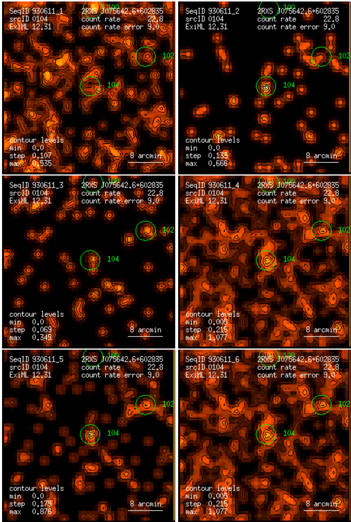
Figure 104: RASS 930611: detection 0104: band rate images, Gaussian filter: (1) PSPC channels 11 – 41, (2) 52 – 90, (3) 91 – 201, (4) 11 – 235, (5) 52 – 201, (6) 11 – 201. Broad band rates in counts/ks. Band rate contour levels in counts/ks/arcmin 2 .
