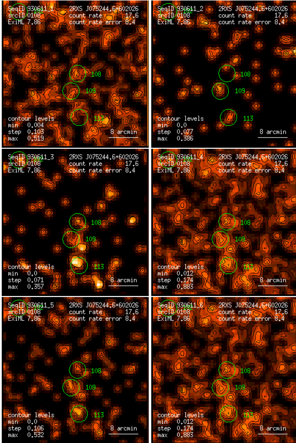
Figure 108: RASS 930611: detection 0108: band rate images, Gaussian filter: (1) PSPC channels 11 – 41, (2) 52 – 90, (3) 91 – 201, (4) 11 – 235, (5) 52 – 201, (6) 11 – 201. Broad band rates in counts/ks. Band rate contour levels in counts/ks/arcmin 2 .
