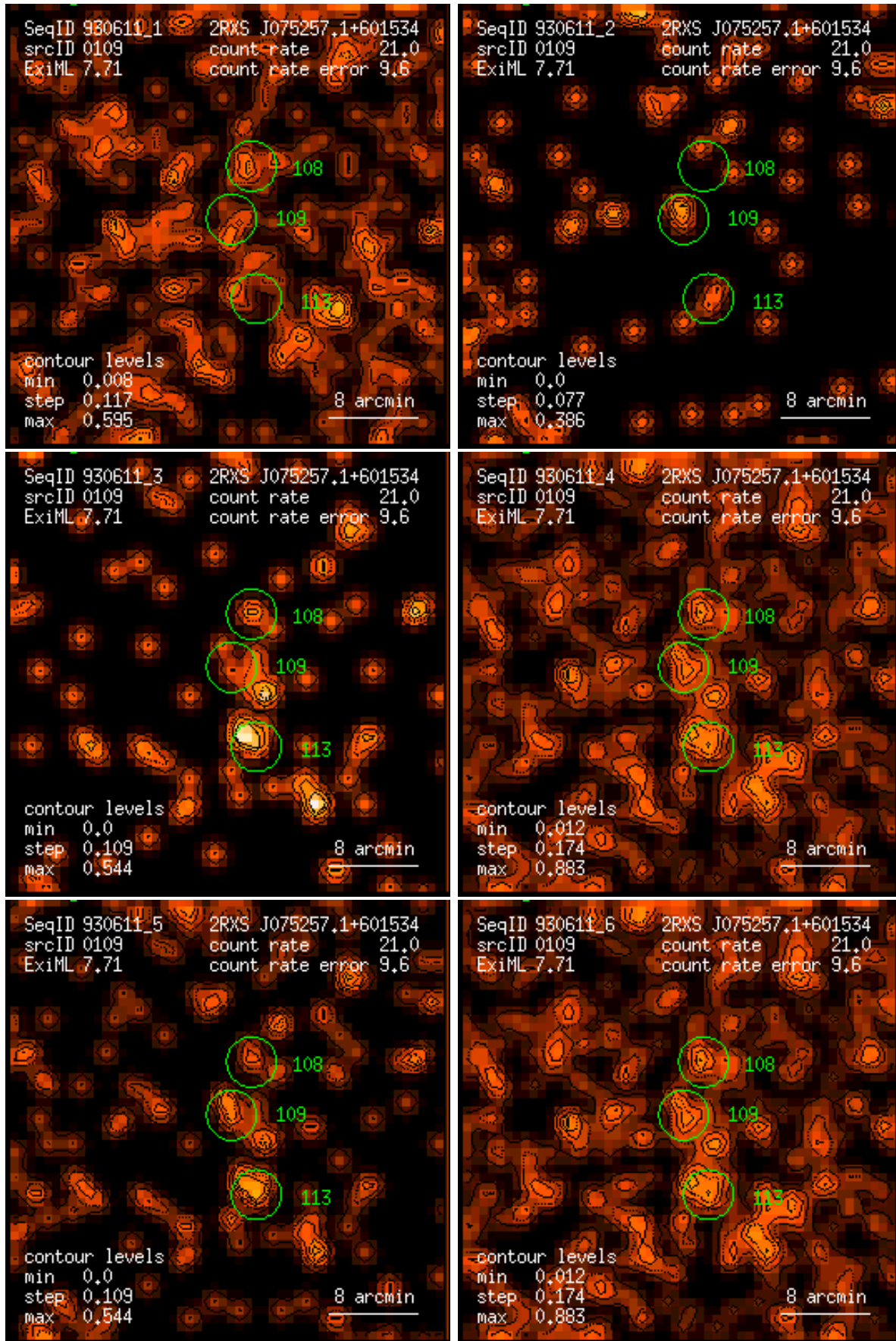
Figure 109: RASS 930611: detection 0109: band rate images, Gaussian filter: (1) PSPC channels 11 – 41, (2) 52 – 90, (3) 91 – 201, (4) 11 – 235, (5) 52 – 201, (6) 11 – 201. Broad band rates in counts/ks. Band rate contour levels in counts/ks/arcmin 2 .
