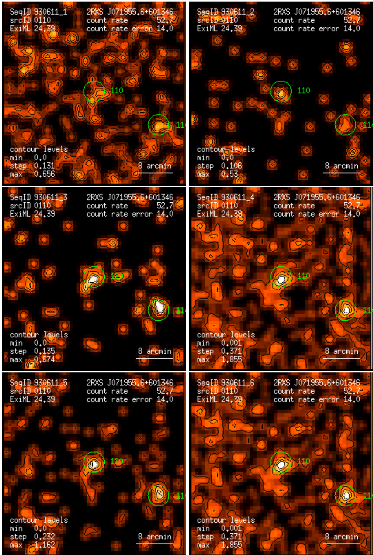
Figure 110: RASS 930611: detection 0110: band rate images, Gaussian filter: (1) PSPC channels 11 – 41, (2) 52 – 90, (3) 91 – 201, (4) 11 – 235, (5) 52 – 201, (6) 11 – 201. Broad band rates in counts/ks. Band rate contour levels in counts/ks/arcmin 2 .
