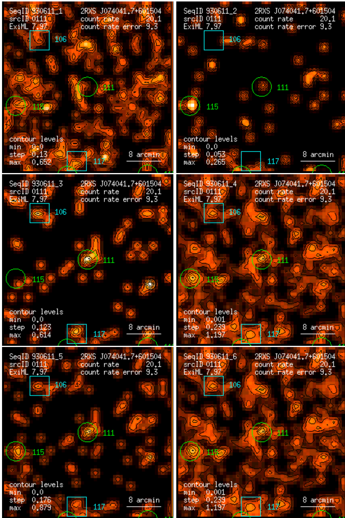
Figure 111: RASS 930611: detection 0111: band rate images, Gaussian filter: (1) PSPC channels 11 – 41, (2) 52 – 90, (3) 91 – 201, (4) 11 – 235, (5) 52 – 201, (6) 11 – 201. Broad band rates in counts/ks. Band rate contour levels in counts/ks/arcmin 2 .
