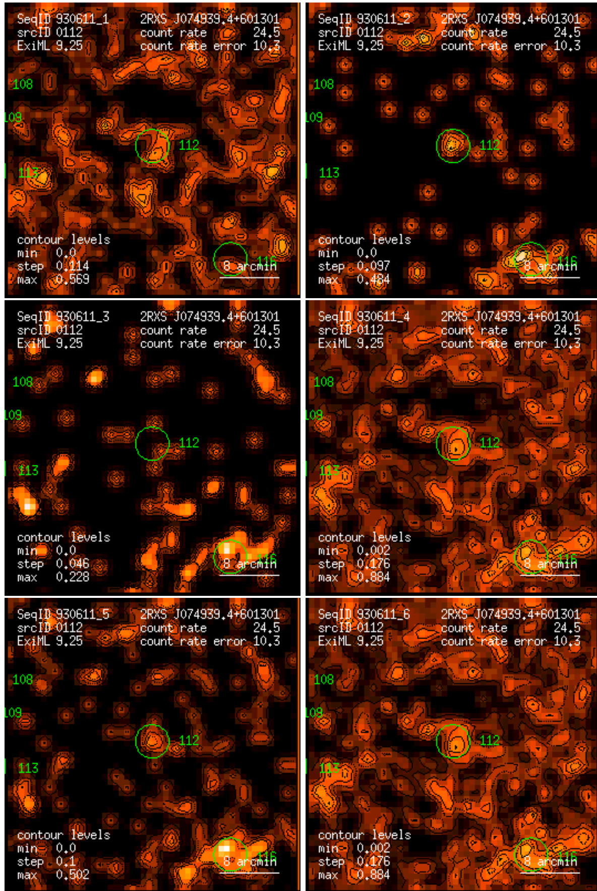
Figure 112: RASS 930611: detection 0112: band rate images, Gaussian filter: (1) PSPC channels 11 – 41, (2) 52 – 90, (3) 91 – 201, (4) 11 – 235, (5) 52 – 201, (6) 11 – 201. Broad band rates in counts/ks. Band rate contour levels in counts/ks/arcmin 2 .
