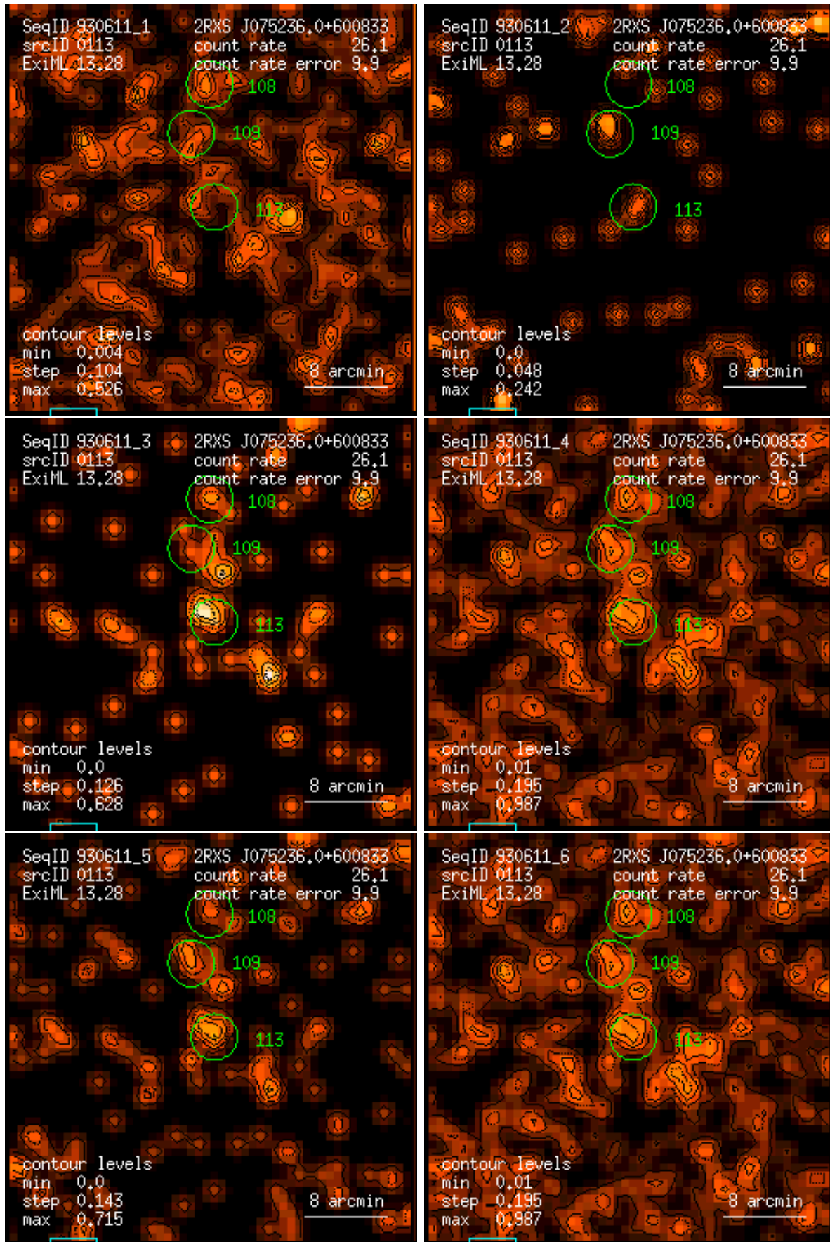
Figure 113: RASS 930611: detection 0113: band rate images, Gaussian filter: (1) PSPC channels 11 – 41, (2) 52 – 90, (3) 91 – 201, (4) 11 – 235, (5) 52 – 201, (6) 11 – 201. Broad band rates in counts/ks. Band rate contour levels in counts/ks/arcmin 2 .
