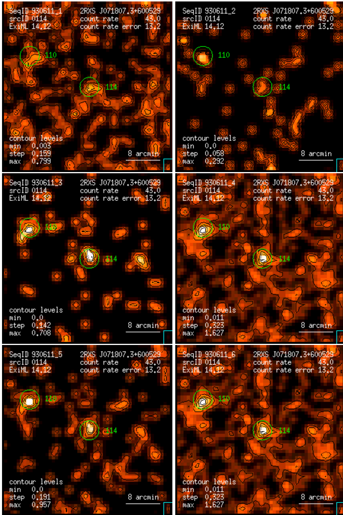
Figure 114: RASS 930611: detection 0114: band rate images, Gaussian filter: (1) PSPC channels 11 – 41, (2) 52 – 90, (3) 91 – 201, (4) 11 – 235, (5) 52 – 201, (6) 11 – 201. Broad band rates in counts/ks. Band rate contour levels in counts/ks/arcmin 2 .
