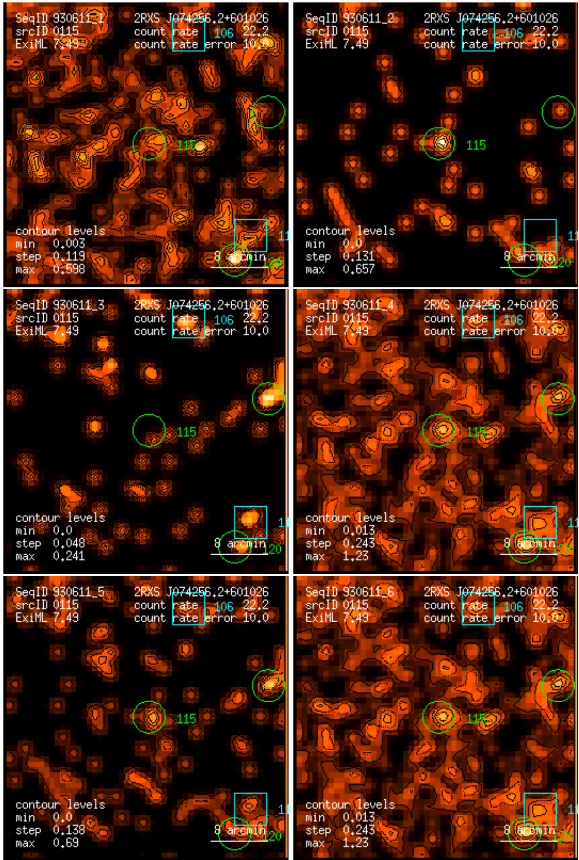
Figure 115: RASS 930611: detection 0115: band rate images, Gaussian filter: (1) PSPC channels 11 – 41, (2) 52 – 90, (3) 91 – 201, (4) 11 – 235, (5) 52 – 201, (6) 11 – 201. Broad band rates in counts/ks. Band rate contour levels in counts/ks/arcmin 2 .
