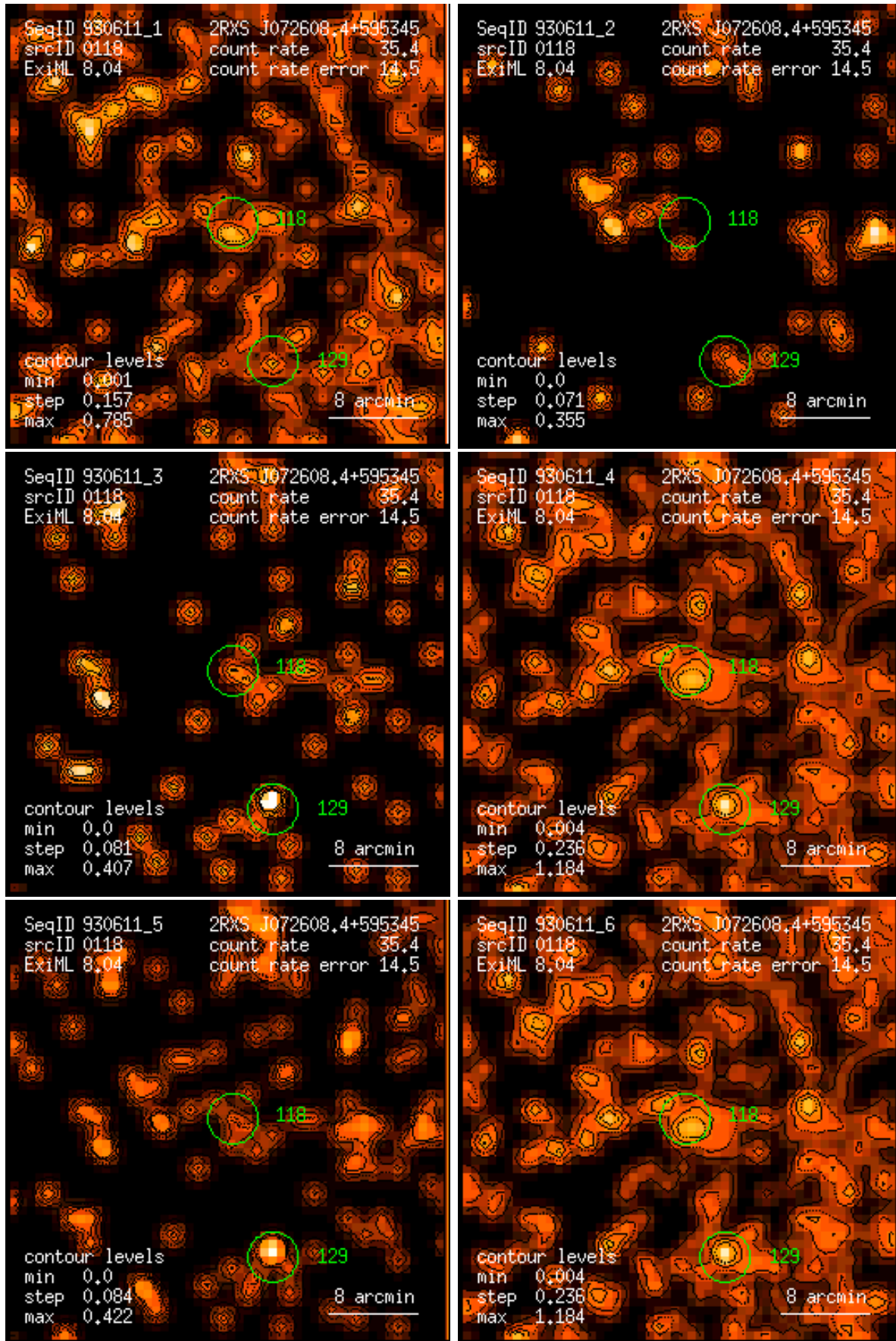
Figure 118: RASS 930611: detection 0118: band rate images, Gaussian filter: (1) PSPC channels 11 – 41, (2) 52 – 90, (3) 91 – 201, (4) 11 – 235, (5) 52 – 201, (6) 11 – 201. Broad band rates in counts/ks. Band rate contour levels in counts/ks/arcmin 2 .
