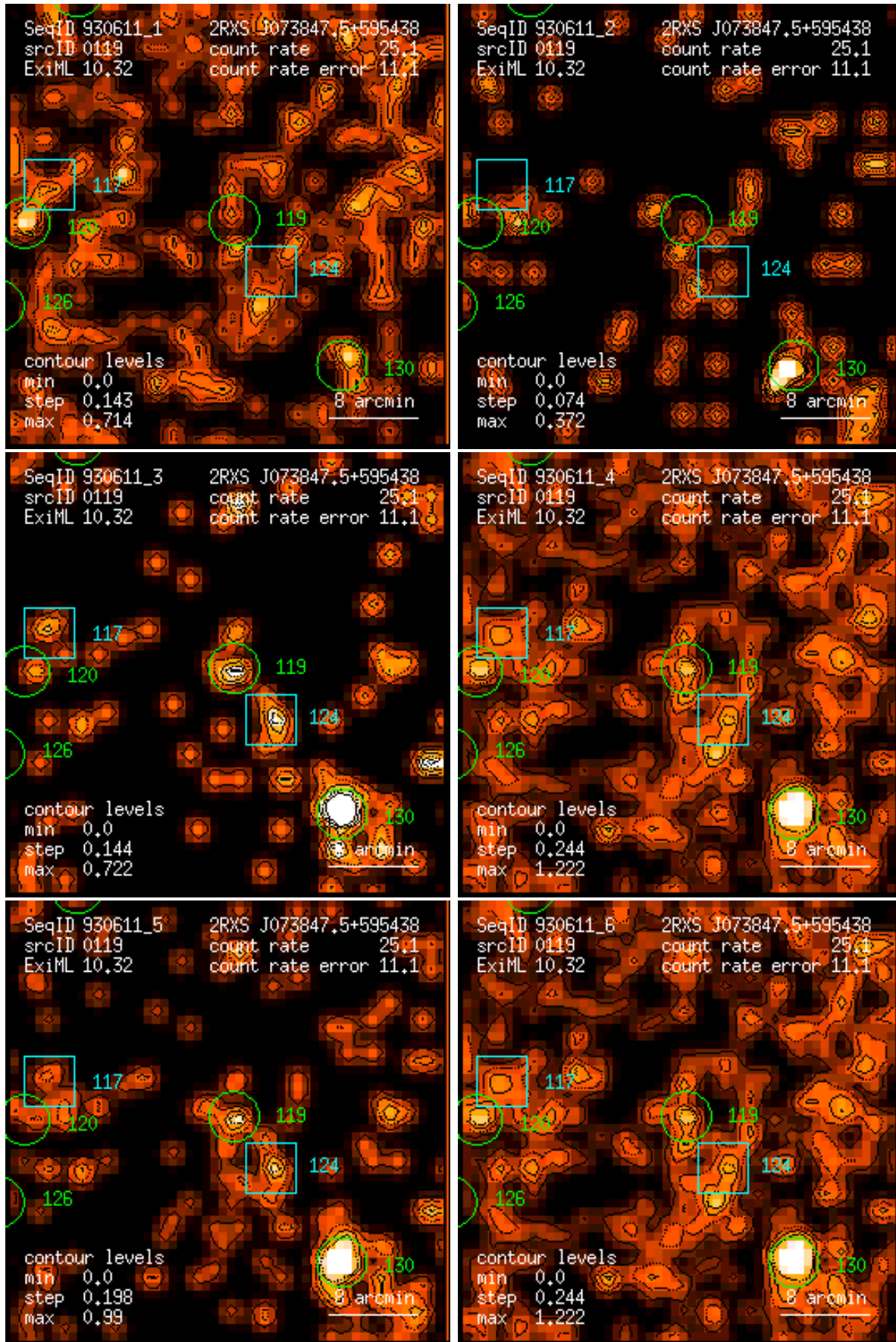
Figure 119: RASS 930611: detection 0119: band rate images, Gaussian filter: (1) PSPC channels 11 – 41, (2) 52 – 90, (3) 91 – 201, (4) 11 – 235, (5) 52 – 201, (6) 11 – 201. Broad band rates in counts/ks. Band rate contour levels in counts/ks/arcmin 2 .
