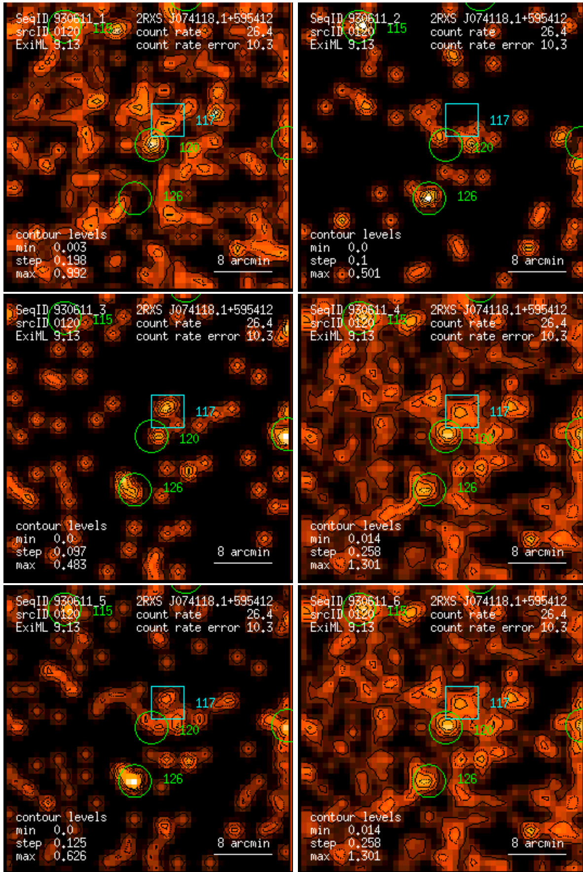
Figure 120: RASS 930611: detection 0120: band rate images, Gaussian filter: (1) PSPC channels 11 – 41, (2) 52 – 90, (3) 91 – 201, (4) 11 – 235, (5) 52 – 201, (6) 11 – 201. Broad band rates in counts/ks. Band rate contour levels in counts/ks/arcmin 2 .
