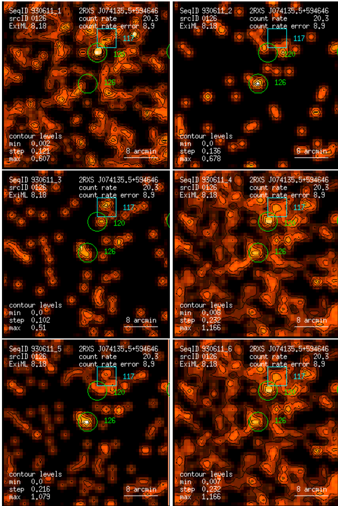
Figure 126: RASS 930611: detection 0126: band rate images, Gaussian filter: (1) PSPC channels 11 – 41, (2) 52 – 90, (3) 91 – 201, (4) 11 – 235, (5) 52 – 201, (6) 11 – 201. Broad band rates in counts/ks. Band rate contour levels in counts/ks/arcmin 2 .
