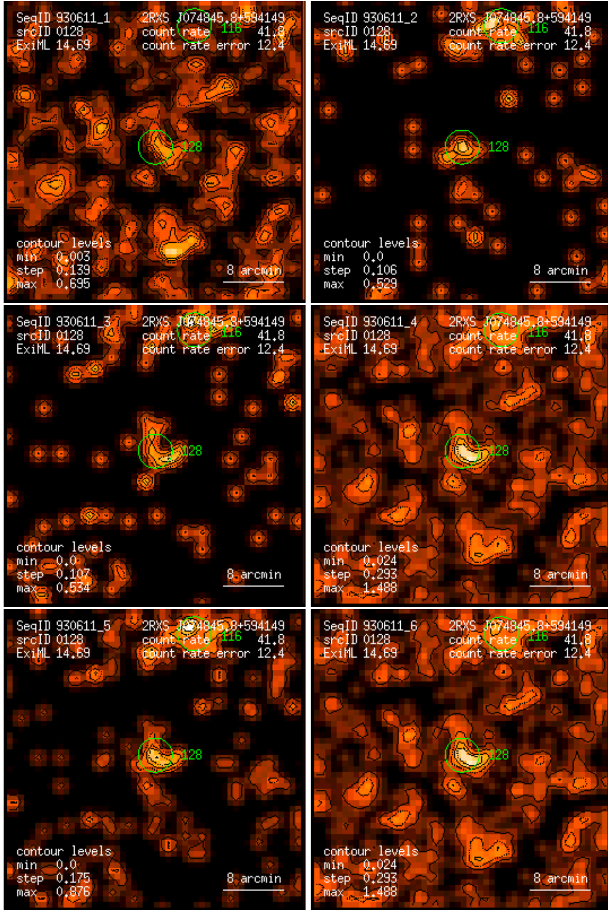
Figure 128: RASS 930611: detection 0128: band rate images, Gaussian filter: (1) PSPC channels 11 – 41, (2) 52 – 90, (3) 91 – 201, (4) 11 – 235, (5) 52 – 201, (6) 11 – 201. Broad band rates in counts/ks. Band rate contour levels in counts/ks/arcmin 2 .
