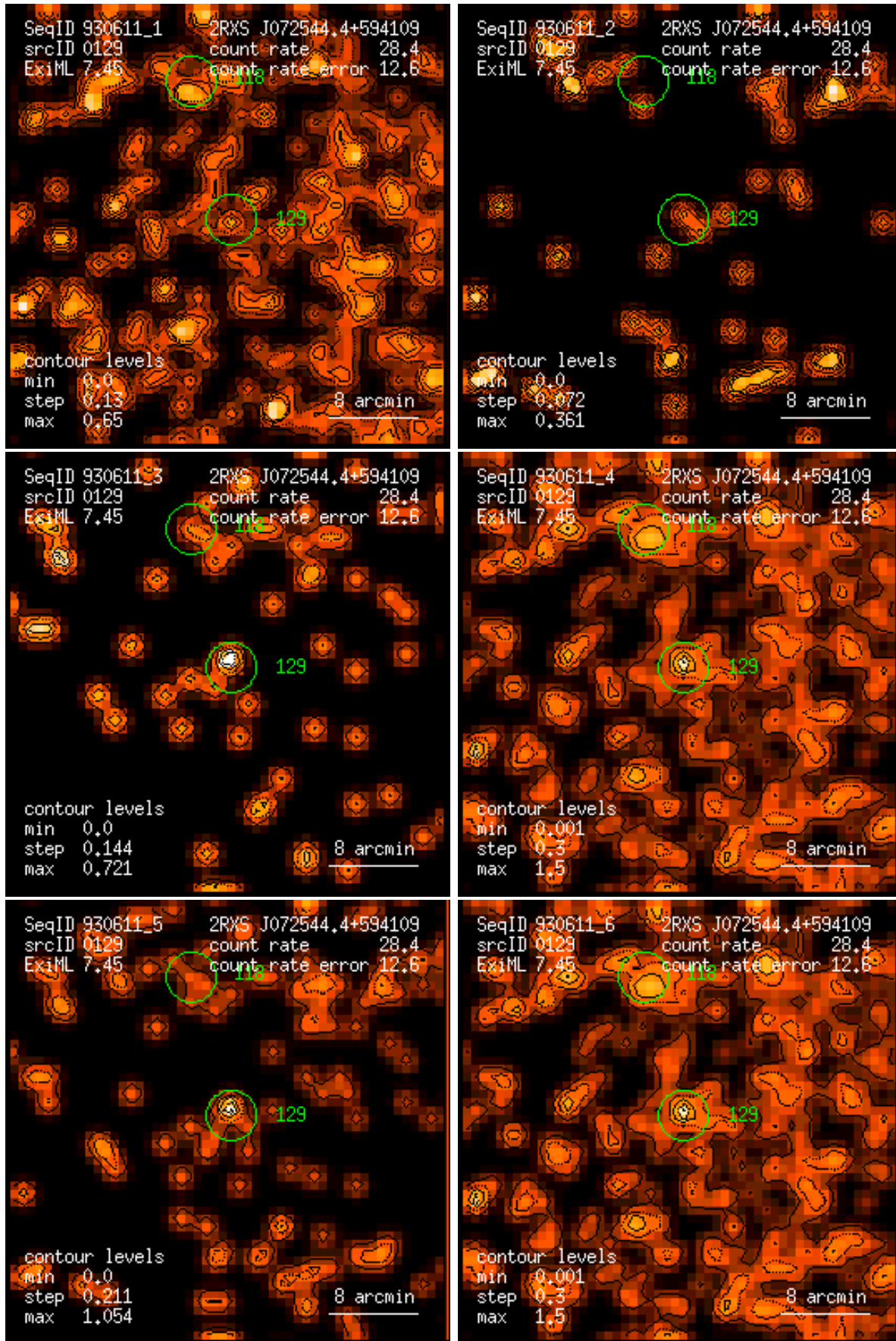
Figure 129: RASS 930611: detection 0129: band rate images, Gaussian filter: (1) PSPC channels 11 – 41, (2) 52 – 90, (3) 91 – 201, (4) 11 – 235, (5) 52 – 201, (6) 11 – 201. Broad band rates in counts/ks. Band rate contour levels in counts/ks/arcmin 2 .
