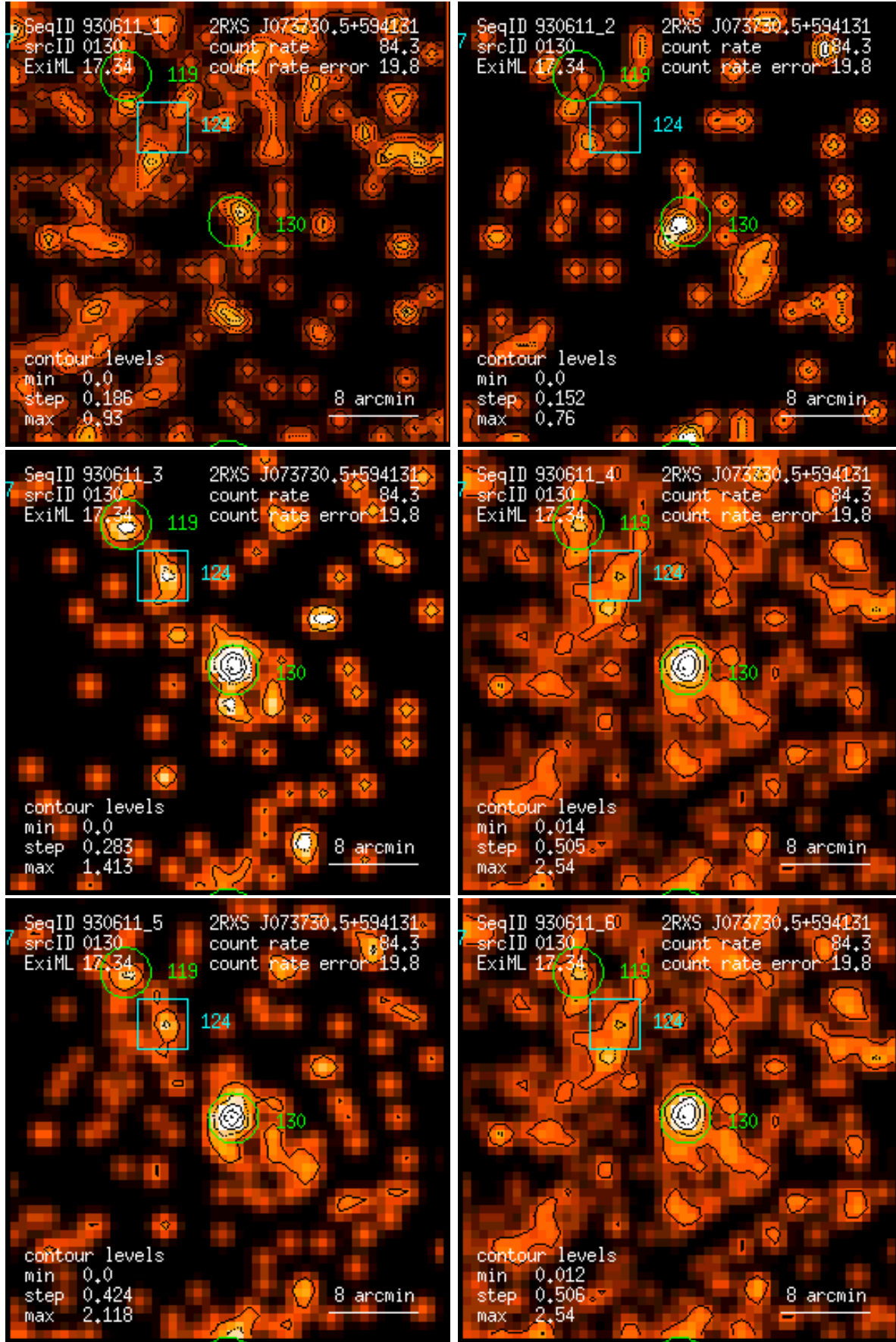
Figure 130: RASS 930611: detection 0130: band rate images, Gaussian filter: (1) PSPC channels 11 – 41, (2) 52 – 90, (3) 91 – 201, (4) 11 – 235, (5) 52 – 201, (6) 11 – 201. Broad band rates in counts/ks. Band rate contour levels in counts/ks/arcmin 2 .
