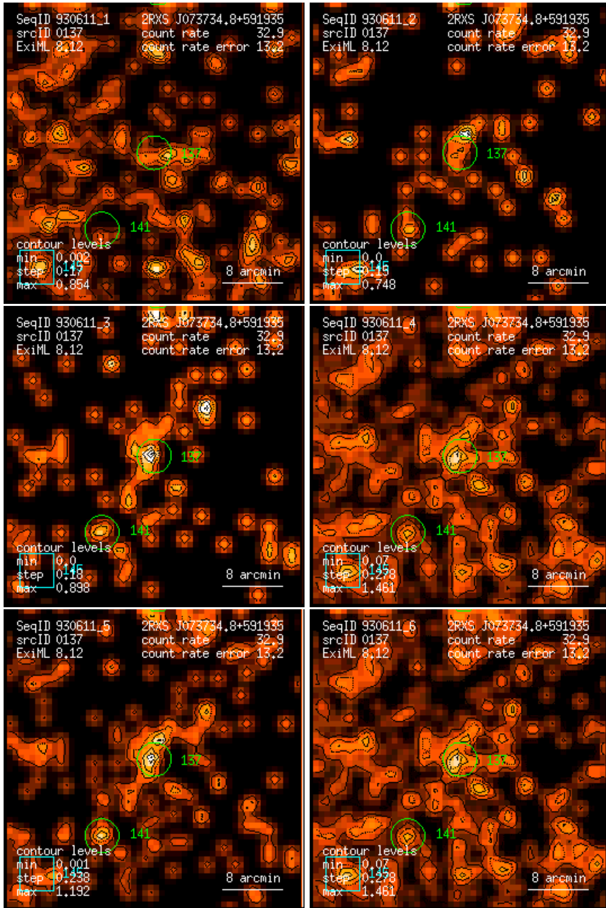
Figure 137: RASS 930611: detection 0137: band rate images, Gaussian filter: (1) PSPC channels 11 – 41, (2) 52 – 90, (3) 91 – 201, (4) 11 – 235, (5) 52 – 201, (6) 11 – 201. Broad band rates in counts/ks. Band rate contour levels in counts/ks/arcmin 2 .
