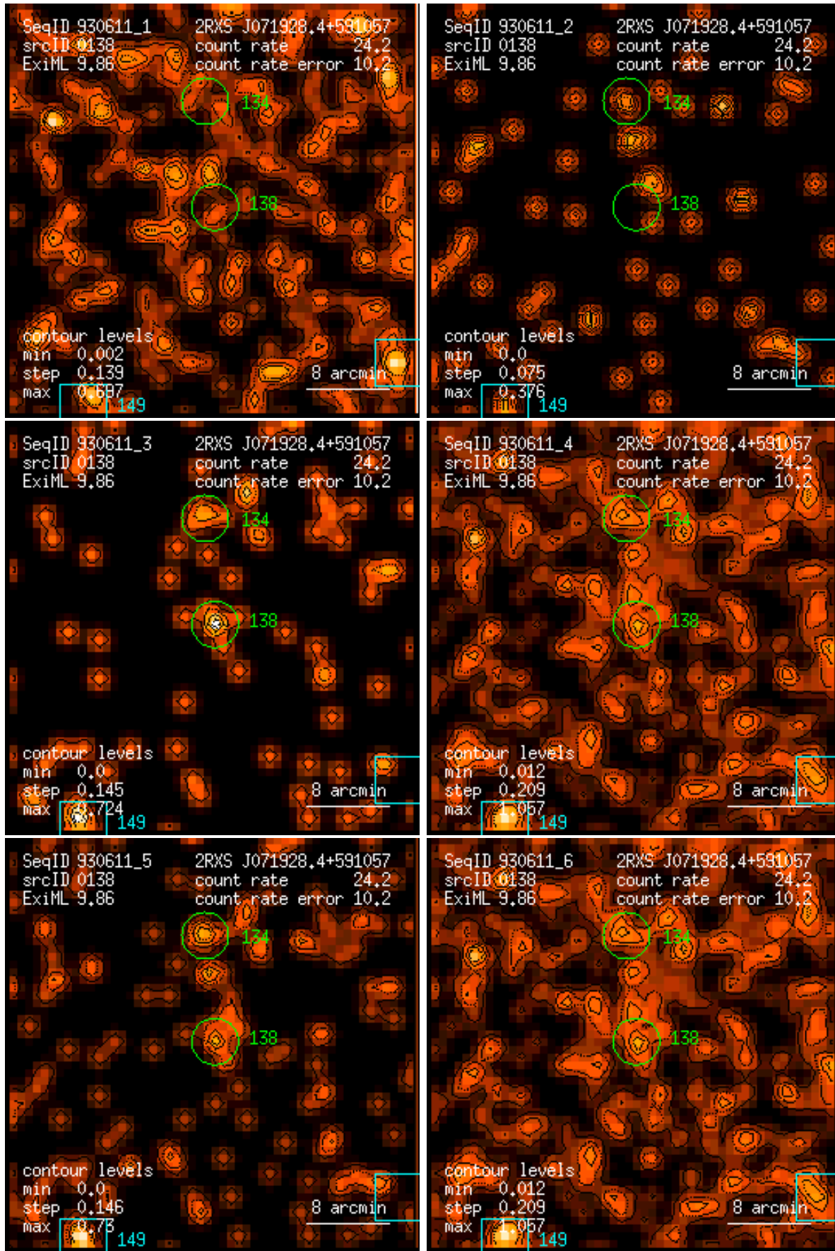
Figure 138: RASS 930611: detection 0138: band rate images, Gaussian filter: (1) PSPC channels 11 – 41, (2) 52 – 90, (3) 91 – 201, (4) 11 – 235, (5) 52 – 201, (6) 11 – 201. Broad band rates in counts/ks. Band rate contour levels in counts/ks/arcmin 2 .
