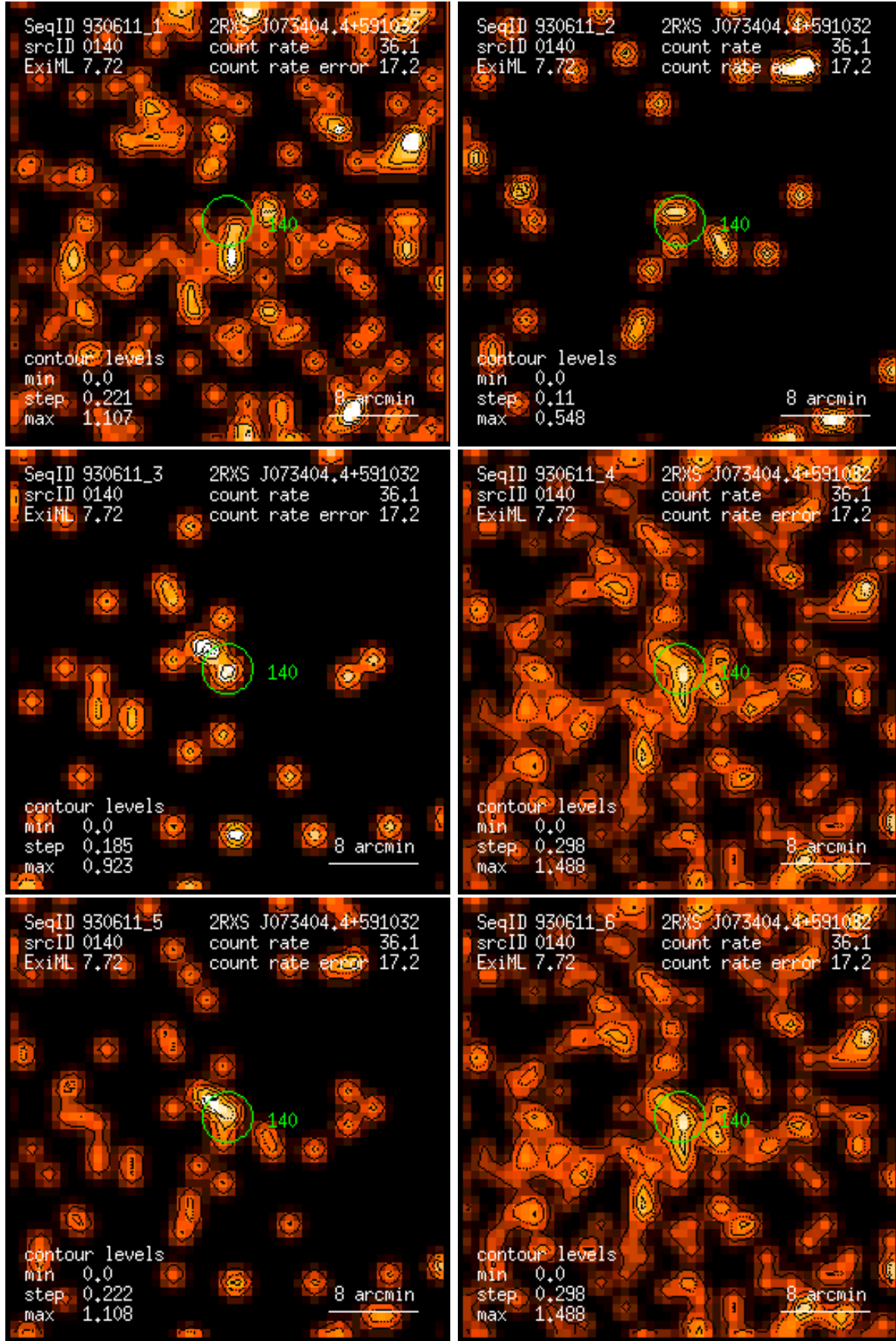
Figure 140: RASS 930611: detection 0140: band rate images, Gaussian filter: (1) PSPC channels 11 – 41, (2) 52 – 90, (3) 91 – 201, (4) 11 – 235, (5) 52 – 201, (6) 11 – 201. Broad band rates in counts/ks. Band rate contour levels in counts/ks/arcmin 2 .
