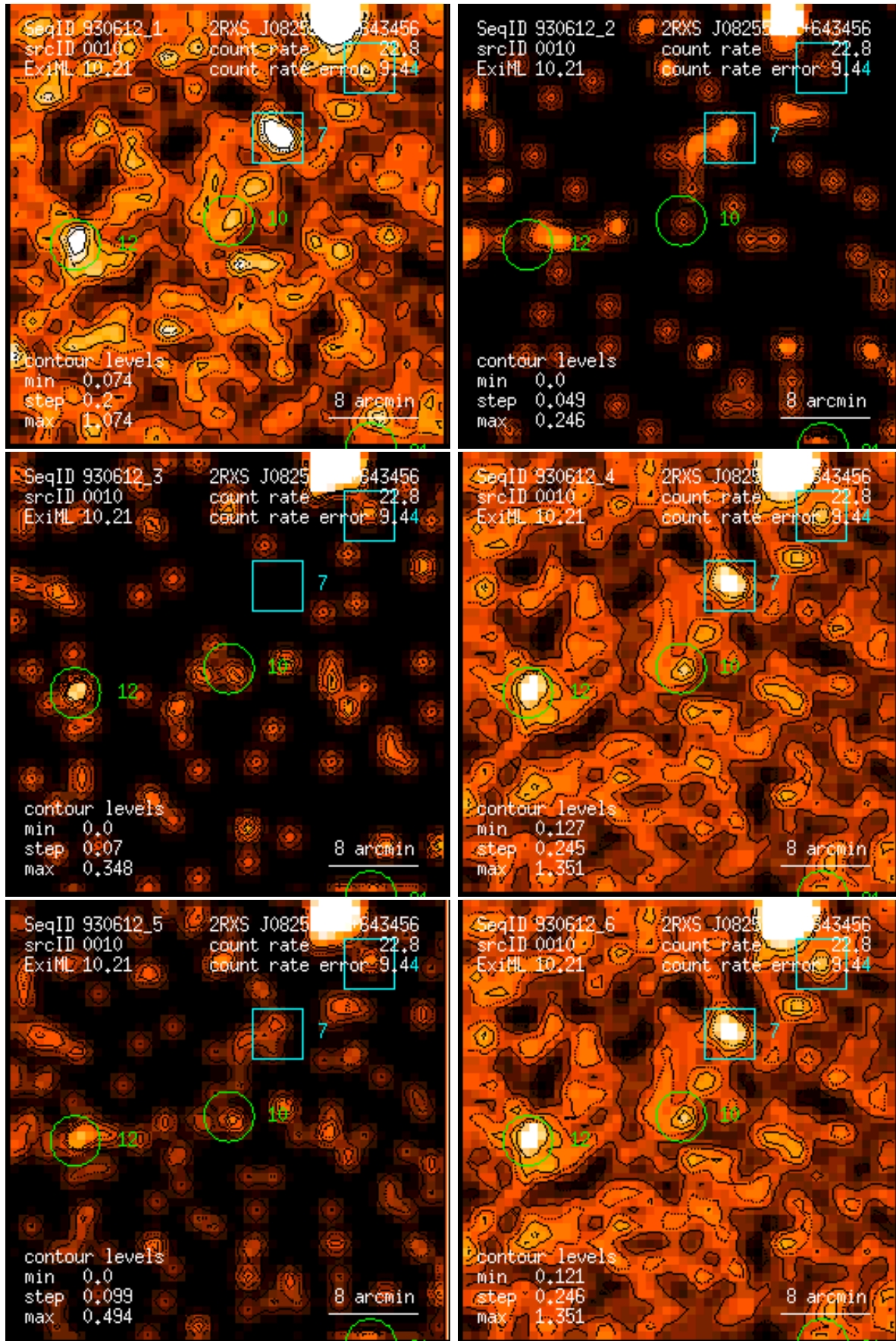
Figure 10: RASS 930612: detection 0010: band rate images, Gaussian filter: (1) PSPC channels 11 – 41, (2) 52 – 90, (3) 91 – 201, (4) 11 – 235, (5) 52 – 201, (6) 11 – 201. Broad band rates in counts/ks. Band rate contour levels in counts/ks/arcmin 2 .
