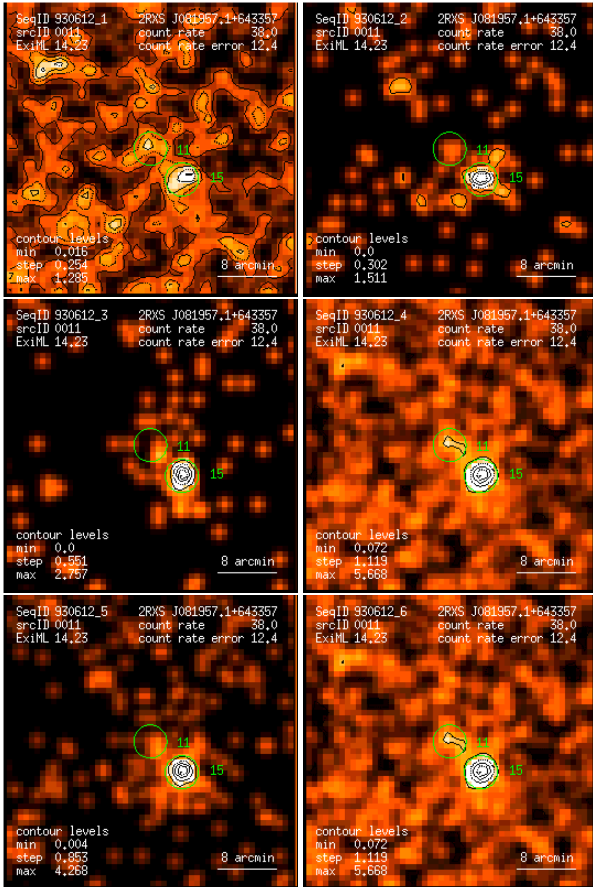
Figure 11: RASS 930612: detection 0011: band rate images, Gaussian filter: (1) PSPC channels 11 – 41, (2) 52 – 90, (3) 91 – 201, (4) 11 – 235, (5) 52 – 201, (6) 11 – 201. Broad band rates in counts/ks. Band rate contour levels in counts/ks/arcmin 2 .
