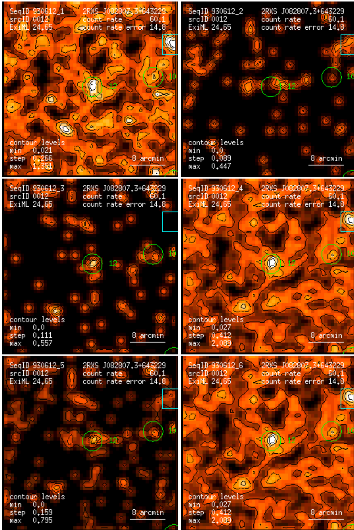
Figure 12: RASS 930612: detection 0012: band rate images, Gaussian filter: (1) PSPC channels 11 – 41, (2) 52 – 90, (3) 91 – 201, (4) 11 – 235, (5) 52 – 201, (6) 11 – 201. Broad band rates in counts/ks. Band rate contour levels in counts/ks/arcmin 2 .
