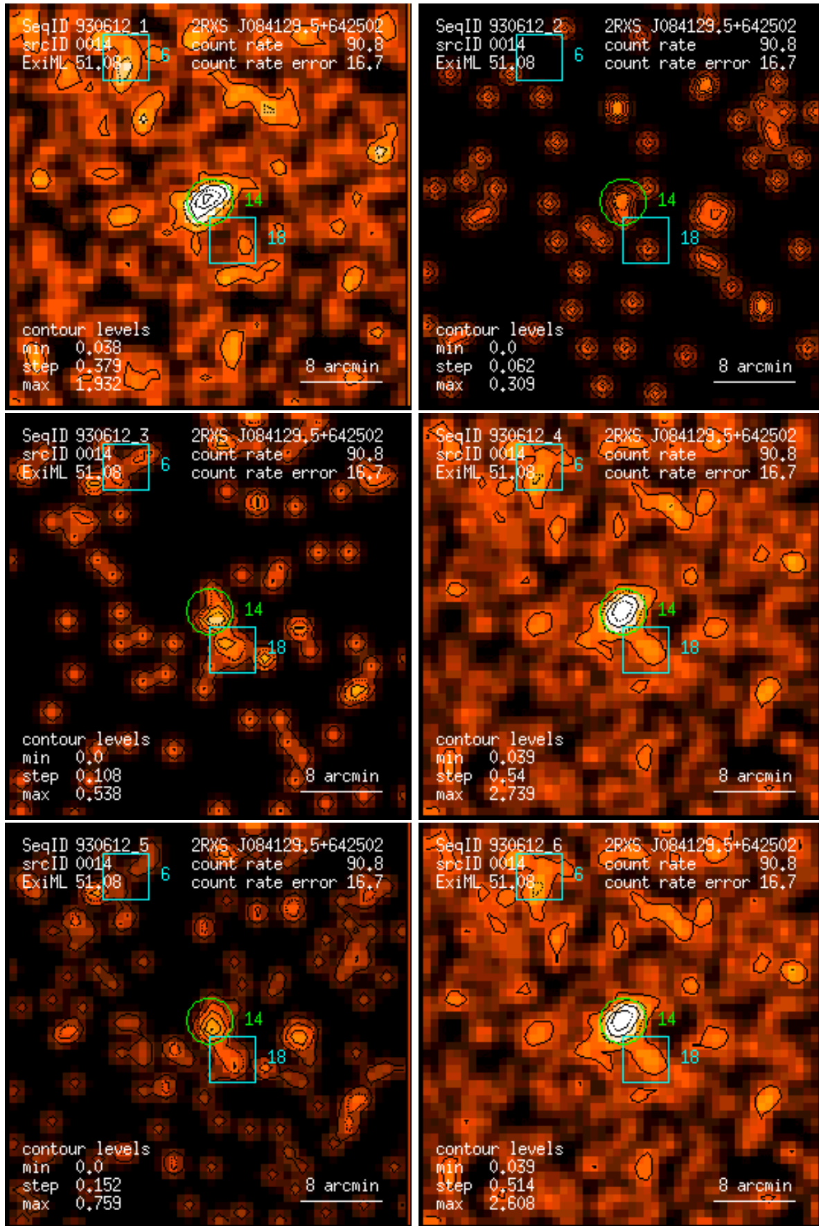
Figure 14: RASS 930612: detection 0014: band rate images, Gaussian filter: (1) PSPC channels 11 – 41, (2) 52 – 90, (3) 91 – 201, (4) 11 – 235, (5) 52 – 201, (6) 11 – 201. Broad band rates in counts/ks. Band rate contour levels in counts/ks/arcmin 2 .
