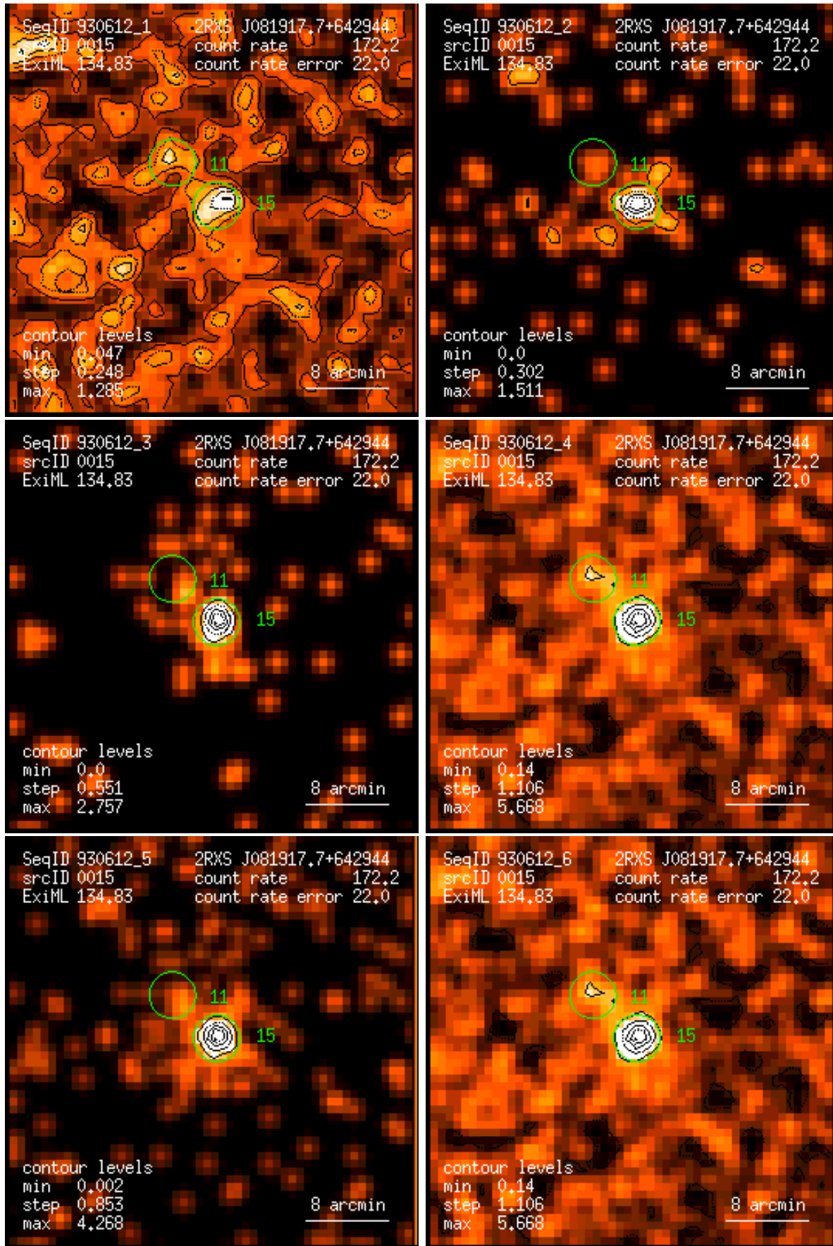
Figure 15: RASS 930612: detection 0015: band rate images, Gaussian filter: (1) PSPC channels 11 – 41, (2) 52 – 90, (3) 91 – 201, (4) 11 – 235, (5) 52 – 201, (6) 11 – 201. Broad band rates in counts/ks. Band rate contour levels in counts/ks/arcmin 2 .
