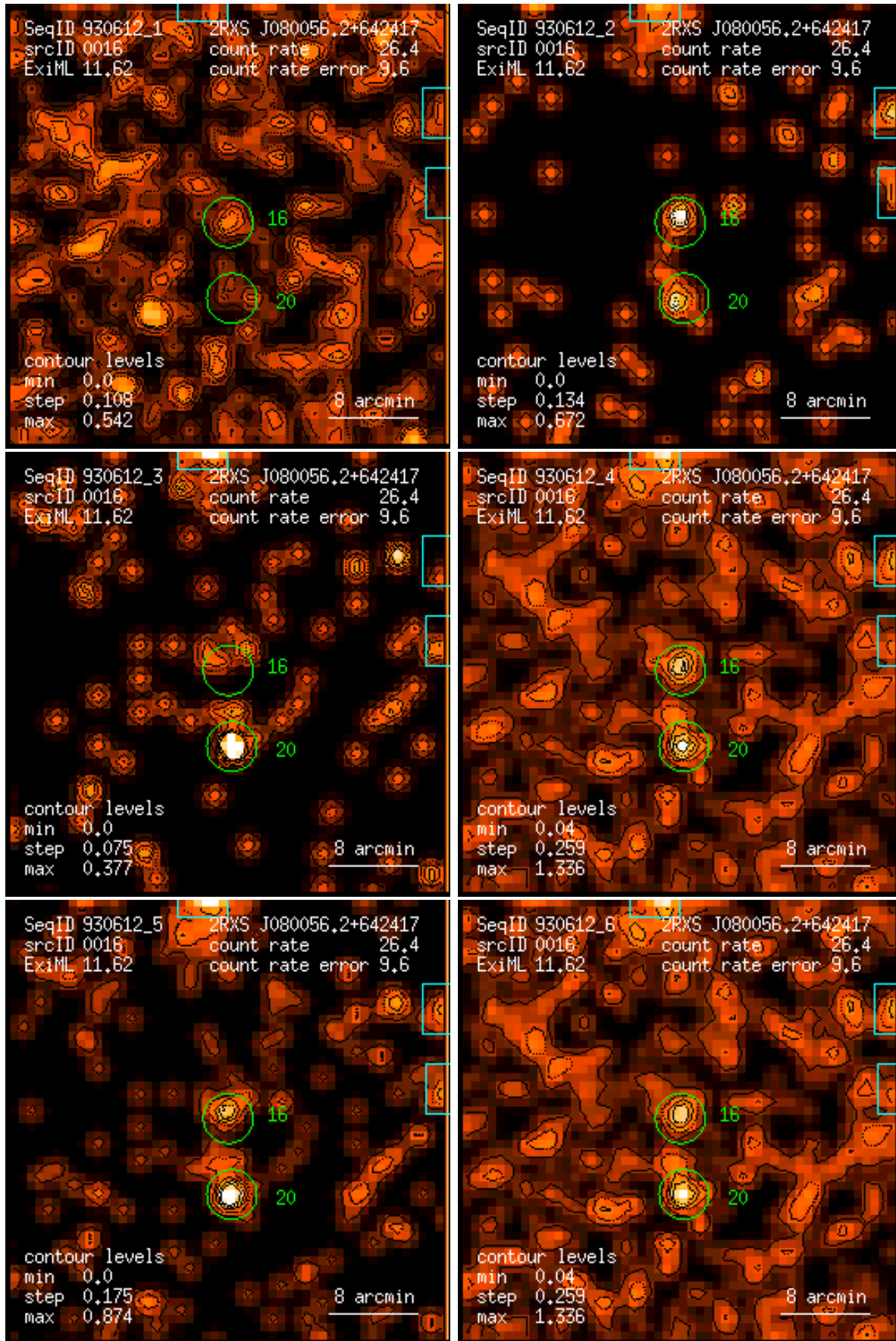
Figure 16: RASS 930612: detection 0016: band rate images, Gaussian filter: (1) PSPC channels 11 – 41, (2) 52 – 90, (3) 91 – 201, (4) 11 – 235, (5) 52 – 201, (6) 11 – 201. Broad band rates in counts/ks. Band rate contour levels in counts/ks/arcmin 2 .
