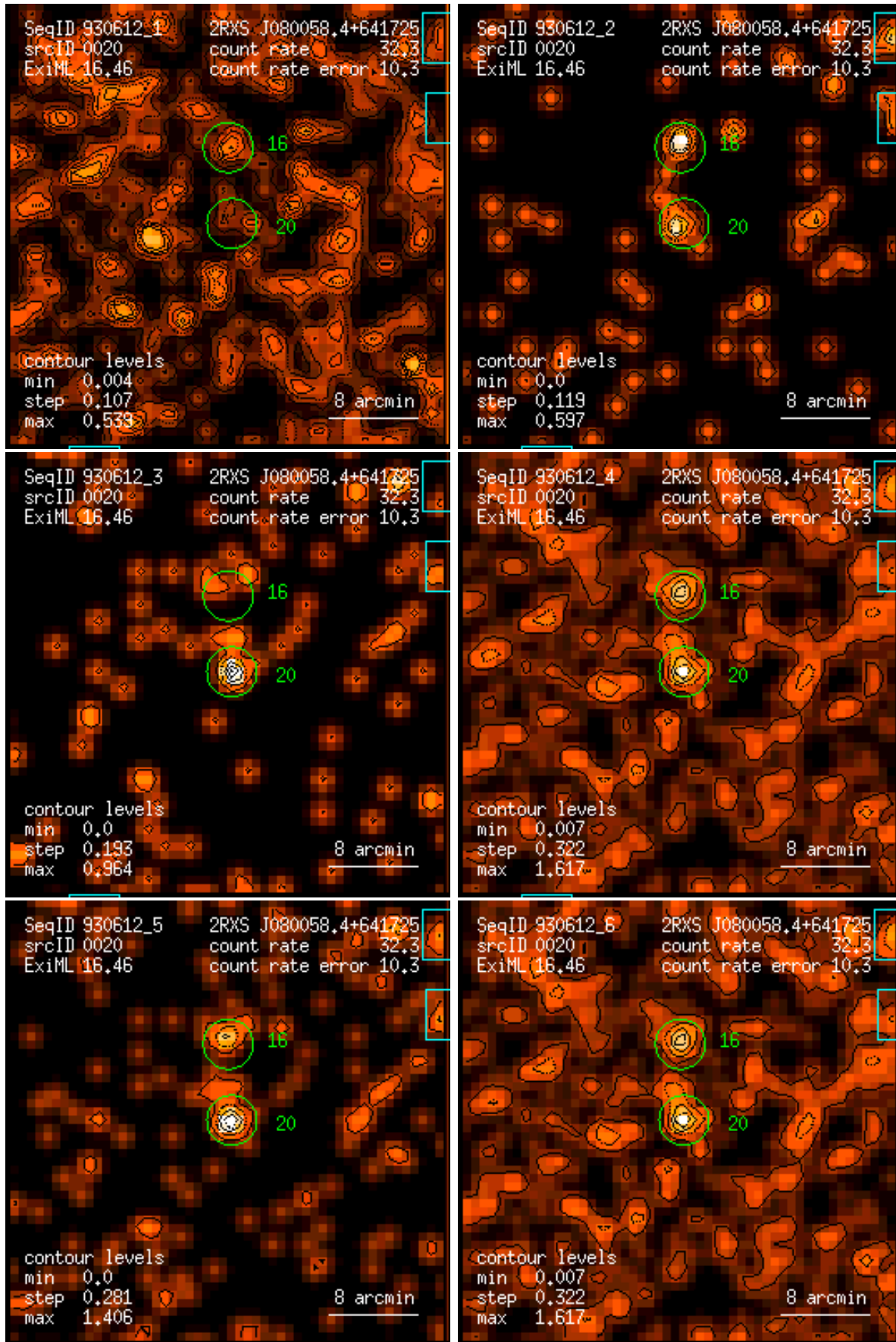
Figure 20: RASS 930612: detection 0020: band rate images, Gaussian filter: (1) PSPC channels 11 – 41, (2) 52 – 90, (3) 91 – 201, (4) 11 – 235, (5) 52 – 201, (6) 11 – 201. Broad band rates in counts/ks. Band rate contour levels in counts/ks/arcmin 2 .
