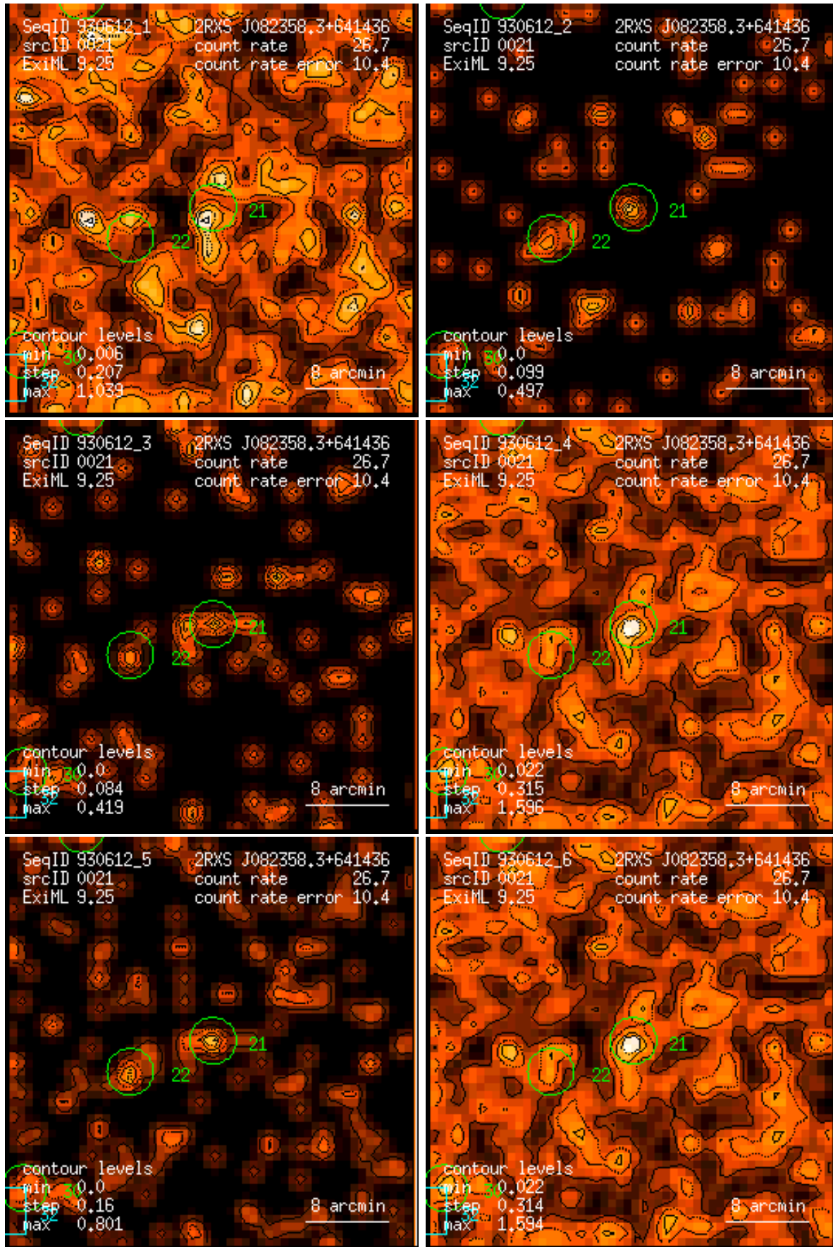
Figure 21: RASS 930612: detection 0021: band rate images, Gaussian filter: (1) PSPC channels 11 – 41, (2) 52 – 90, (3) 91 – 201, (4) 11 – 235, (5) 52 – 201, (6) 11 – 201. Broad band rates in counts/ks. Band rate contour levels in counts/ks/arcmin 2 .
