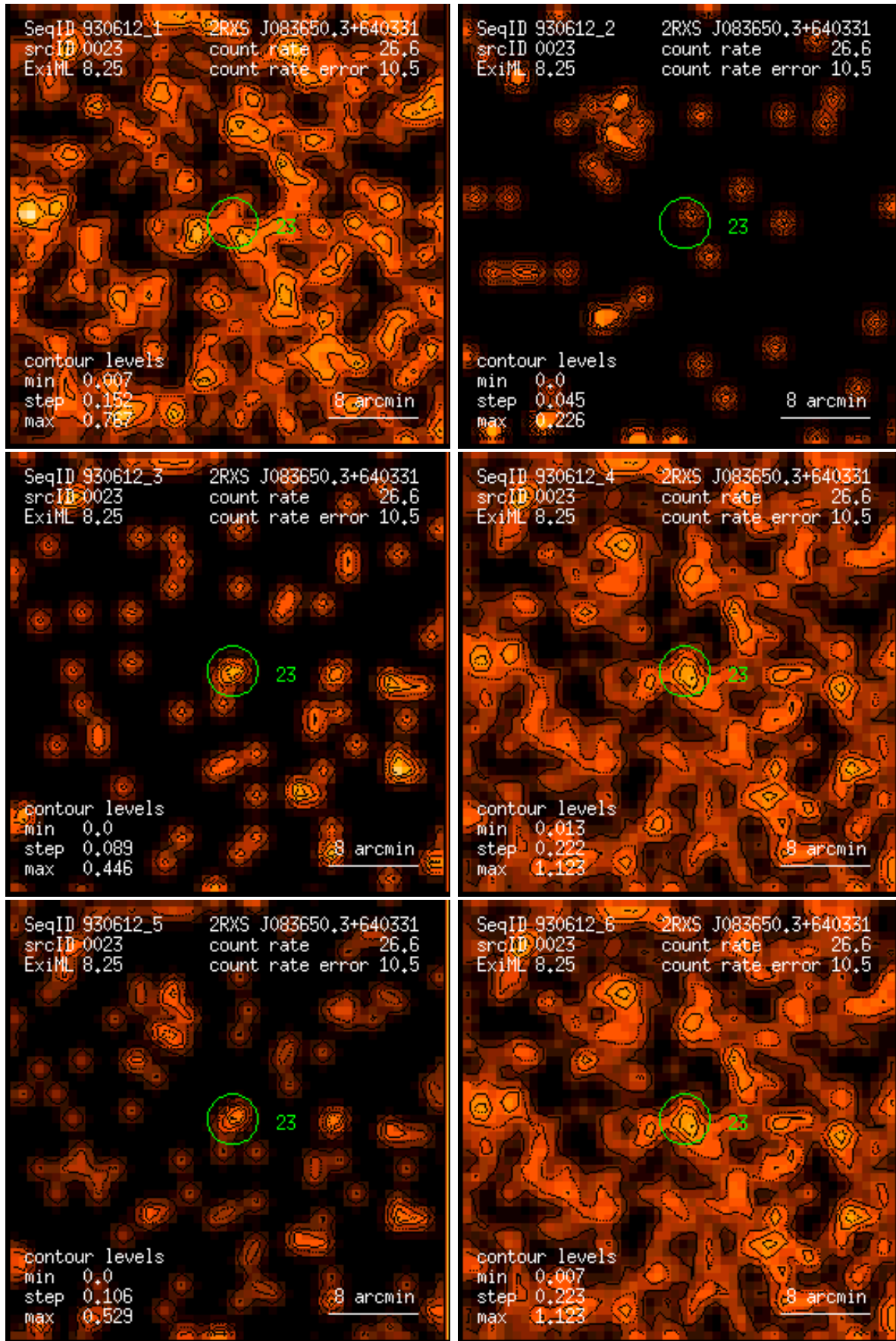
Figure 23: RASS 930612: detection 0023: band rate images, Gaussian filter: (1) PSPC channels 11 – 41, (2) 52 – 90, (3) 91 – 201, (4) 11 – 235, (5) 52 – 201, (6) 11 – 201. Broad band rates in counts/ks. Band rate contour levels in counts/ks/arcmin 2 .
