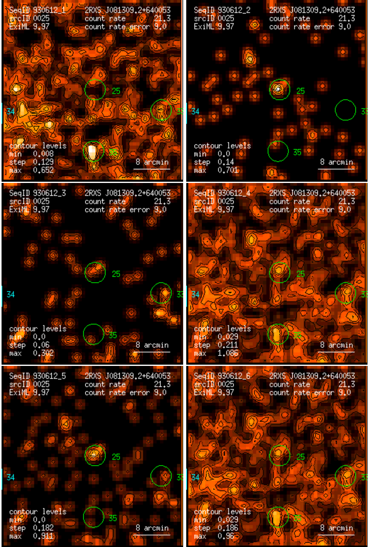
Figure 25: RASS 930612: detection 0025: band rate images, Gaussian filter: (1) PSPC channels 11 – 41, (2) 52 – 90, (3) 91 – 201, (4) 11 – 235, (5) 52 – 201, (6) 11 – 201. Broad band rates in counts/ks. Band rate contour levels in counts/ks/arcmin 2 .
