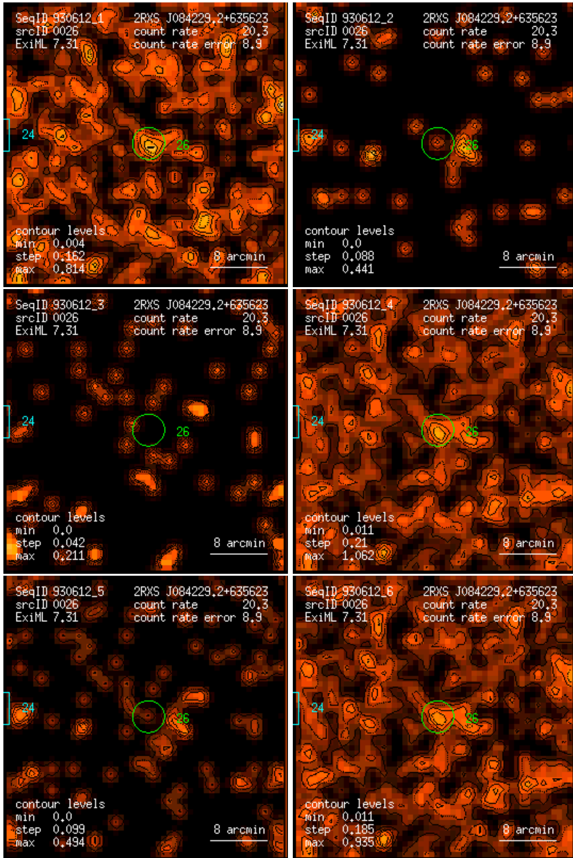
Figure 26: RASS 930612: detection 0026: band rate images, Gaussian filter: (1) PSPC channels 11 – 41, (2) 52 – 90, (3) 91 – 201, (4) 11 – 235, (5) 52 – 201, (6) 11 – 201. Broad band rates in counts/ks. Band rate contour levels in counts/ks/arcmin 2 .
