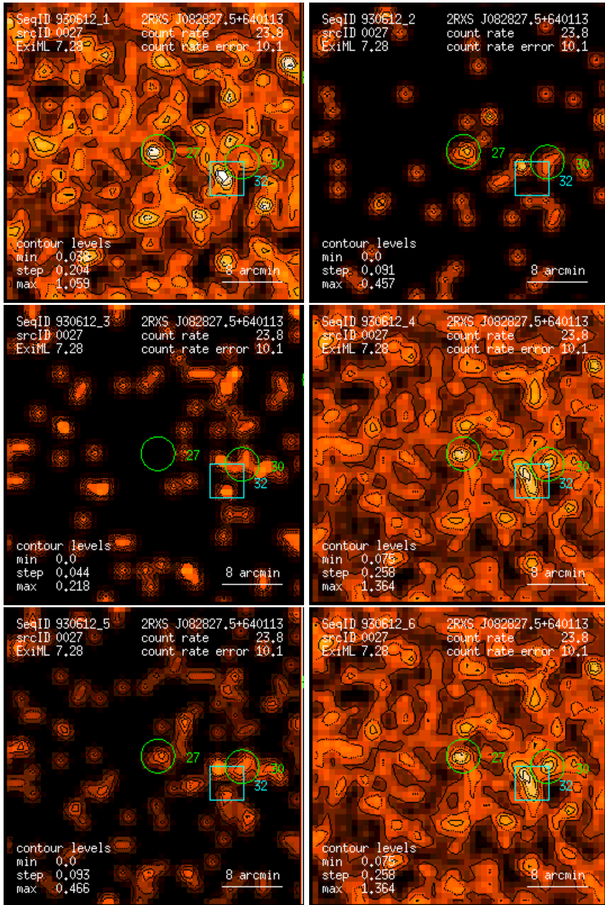
Figure 27: RASS 930612: detection 0027: band rate images, Gaussian filter: (1) PSPC channels 11 – 41, (2) 52 – 90, (3) 91 – 201, (4) 11 – 235, (5) 52 – 201, (6) 11 – 201. Broad band rates in counts/ks. Band rate contour levels in counts/ks/arcmin 2 .
