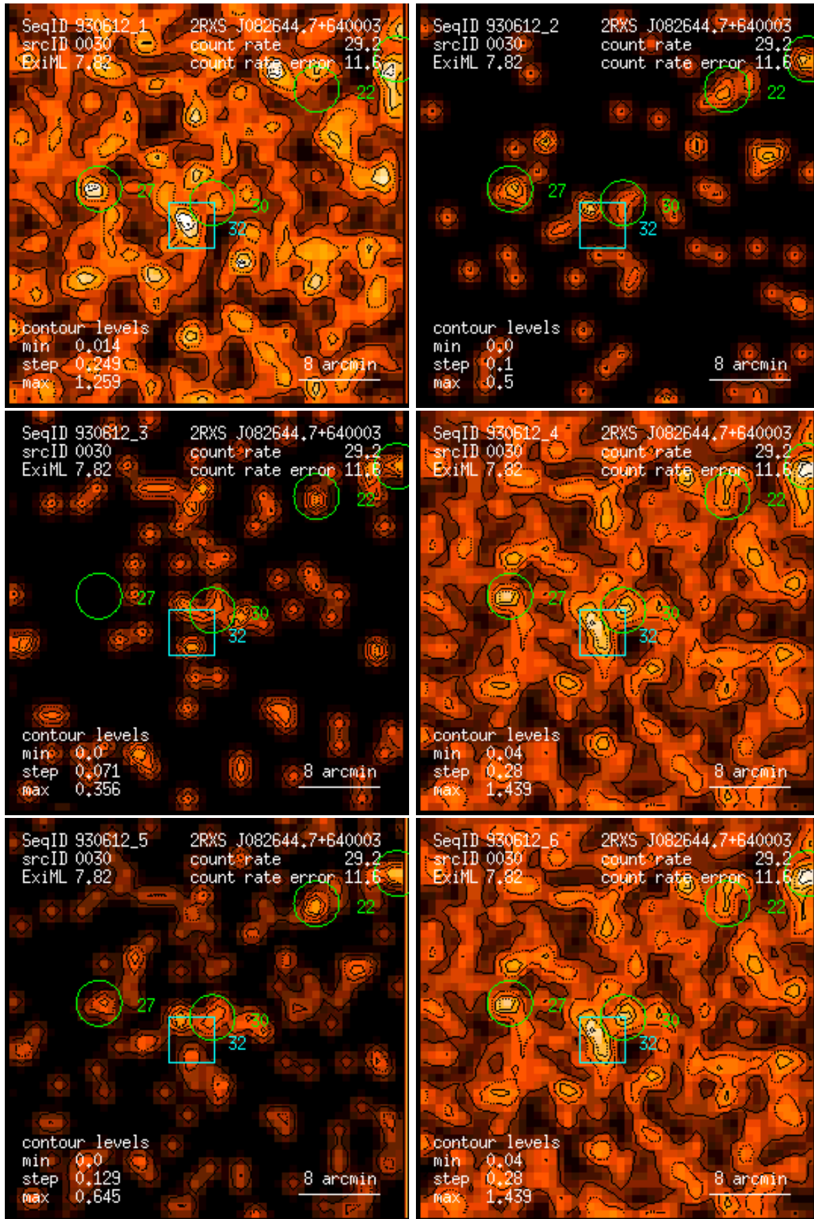
Figure 30: RASS 930612: detection 0030: band rate images, Gaussian filter: (1) PSPC channels 11 – 41, (2) 52 – 90, (3) 91 – 201, (4) 11 – 235, (5) 52 – 201, (6) 11 – 201. Broad band rates in counts/ks. Band rate contour levels in counts/ks/arcmin 2 .
