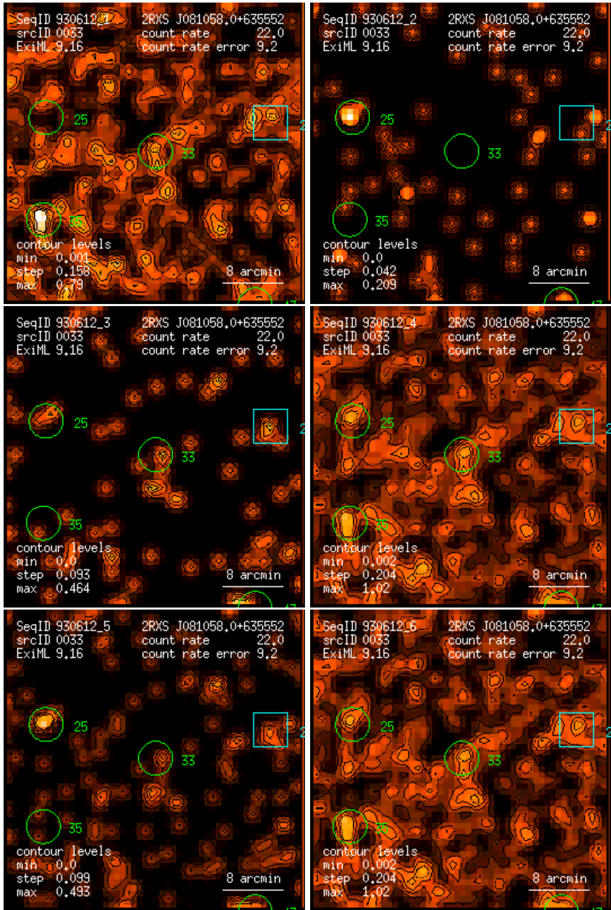
Figure 33: RASS 930612: detection 0033: band rate images, Gaussian filter: (1) PSPC channels 11 – 41, (2) 52 – 90, (3) 91 – 201, (4) 11 – 235, (5) 52 – 201, (6) 11 – 201. Broad band rates in counts/ks. Band rate contour levels in counts/ks/arcmin 2 .
