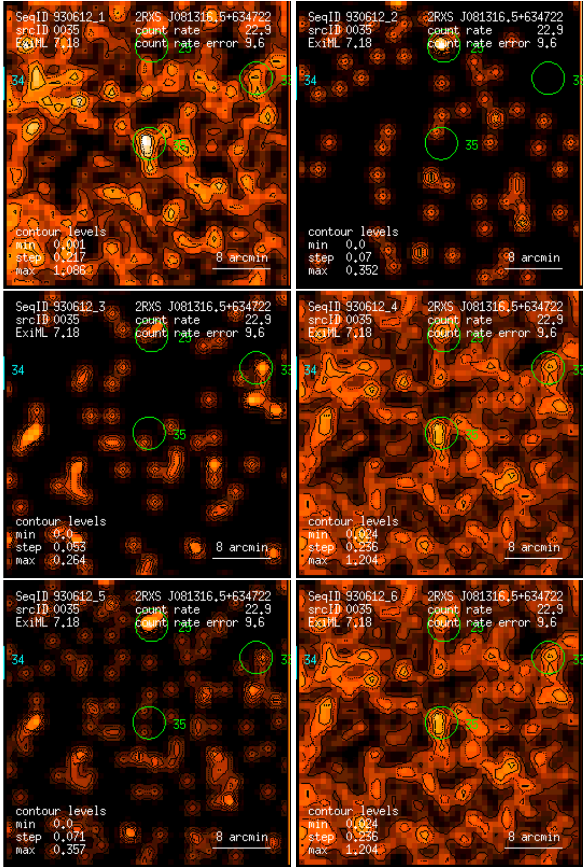
Figure 35: RASS 930612: detection 0035: band rate images, Gaussian filter: (1) PSPC channels 11 – 41, (2) 52 – 90, (3) 91 – 201, (4) 11 – 235, (5) 52 – 201, (6) 11 – 201. Broad band rates in counts/ks. Band rate contour levels in counts/ks/arcmin 2 .
