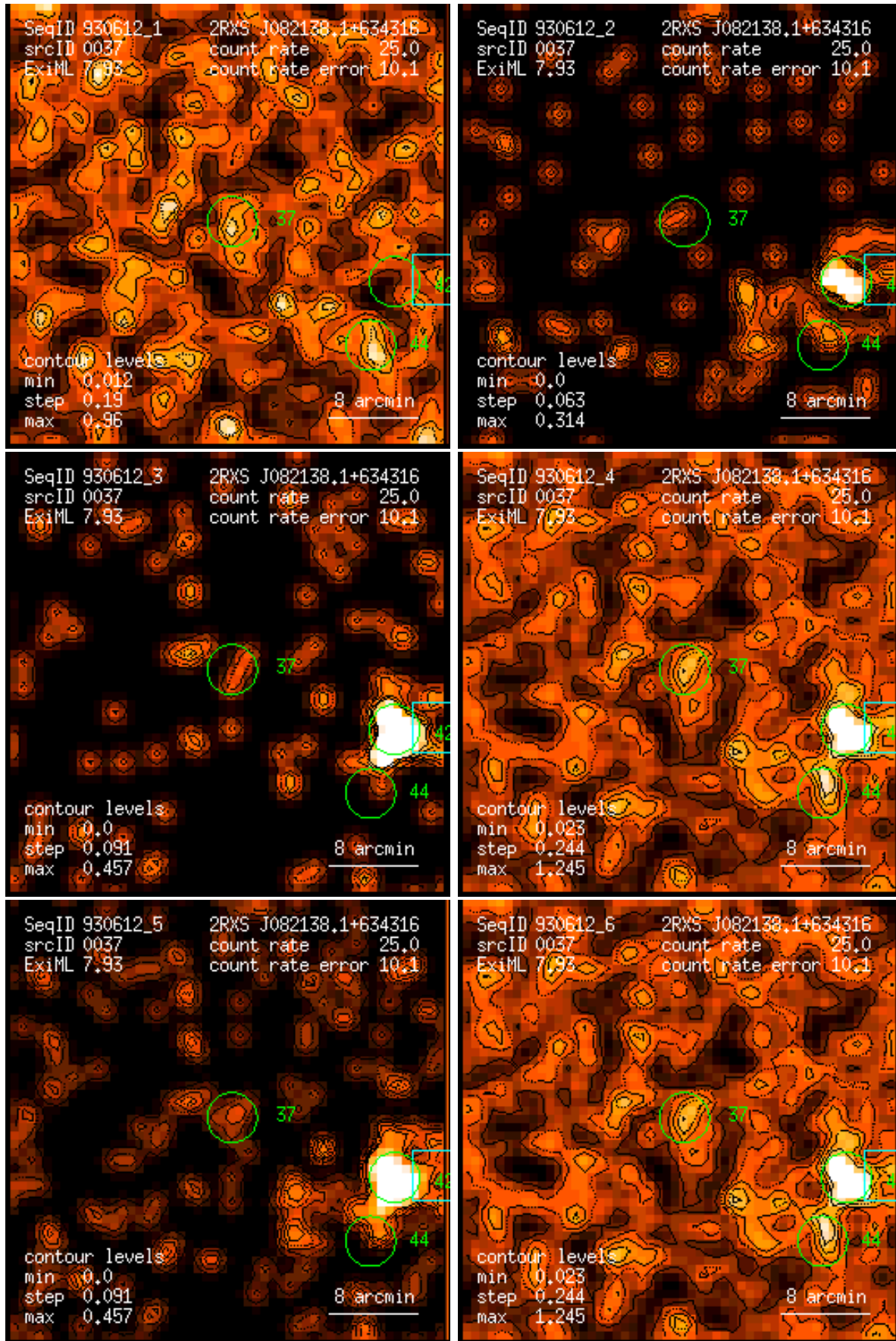
Figure 37: RASS 930612: detection 0037: band rate images, Gaussian filter: (1) PSPC channels 11 – 41, (2) 52 – 90, (3) 91 – 201, (4) 11 – 235, (5) 52 – 201, (6) 11 – 201. Broad band rates in counts/ks. Band rate contour levels in counts/ks/arcmin 2 .
