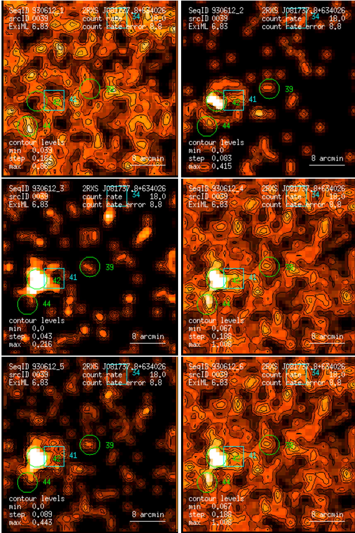
Figure 39: RASS 930612: detection 0039: band rate images, Gaussian filter: (1) PSPC channels 11 – 41, (2) 52 – 90, (3) 91 – 201, (4) 11 – 235, (5) 52 – 201, (6) 11 – 201. Broad band rates in counts/ks. Band rate contour levels in counts/ks/arcmin 2 .
