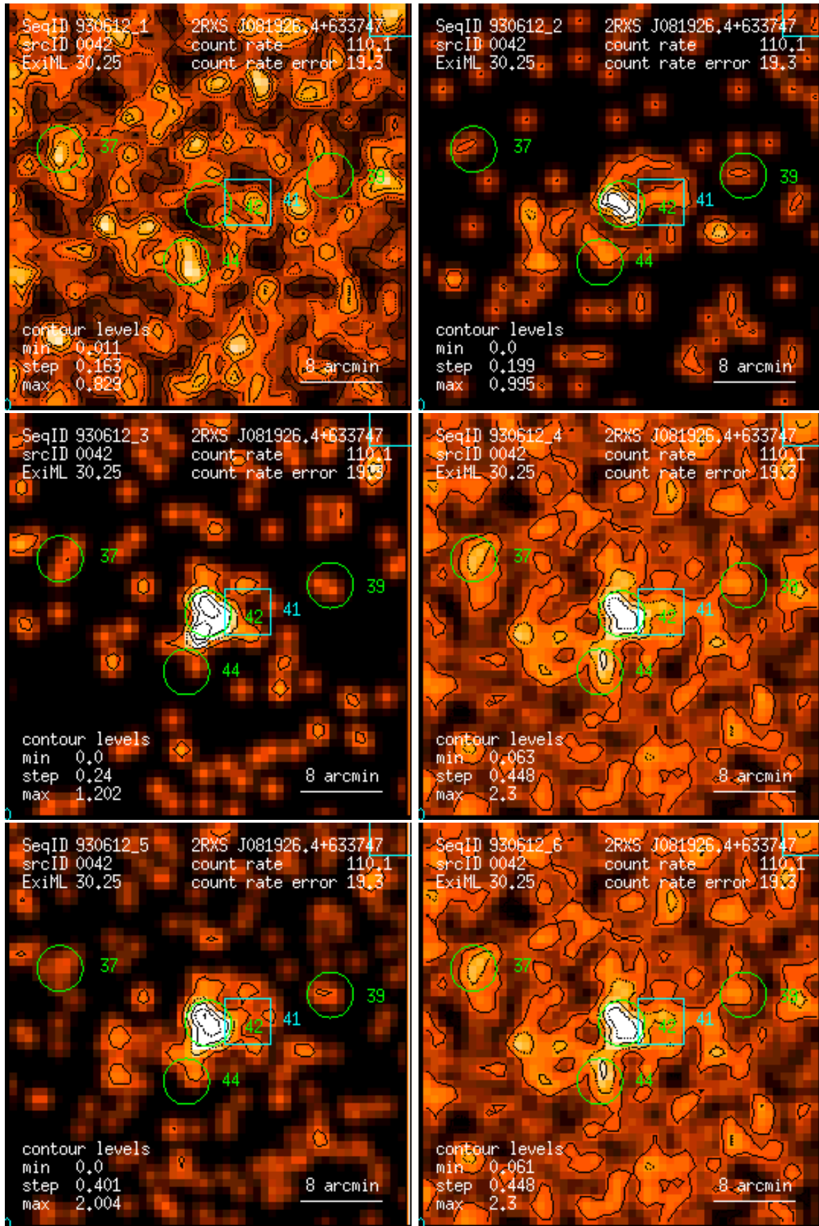
Figure 42: RASS 930612: detection 0042: band rate images, Gaussian filter: (1) PSPC channels 11 – 41, (2) 52 – 90, (3) 91 – 201, (4) 11 – 235, (5) 52 – 201, (6) 11 – 201. Broad band rates in counts/ks. Band rate contour levels in counts/ks/arcmin 2 .
