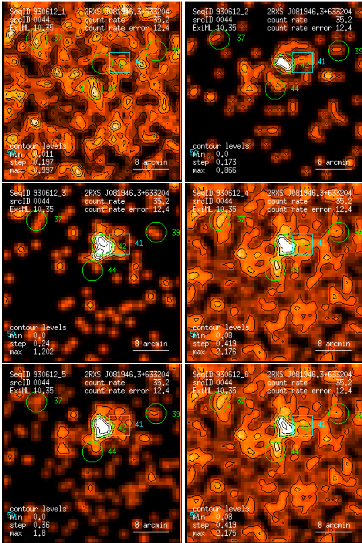
Figure 44: RASS 930612: detection 0044: band rate images, Gaussian filter: (1) PSPC channels 11 – 41, (2) 52 – 90, (3) 91 – 201, (4) 11 – 235, (5) 52 – 201, (6) 11 – 201. Broad band rates in counts/ks. Band rate contour levels in counts/ks/arcmin 2 .
