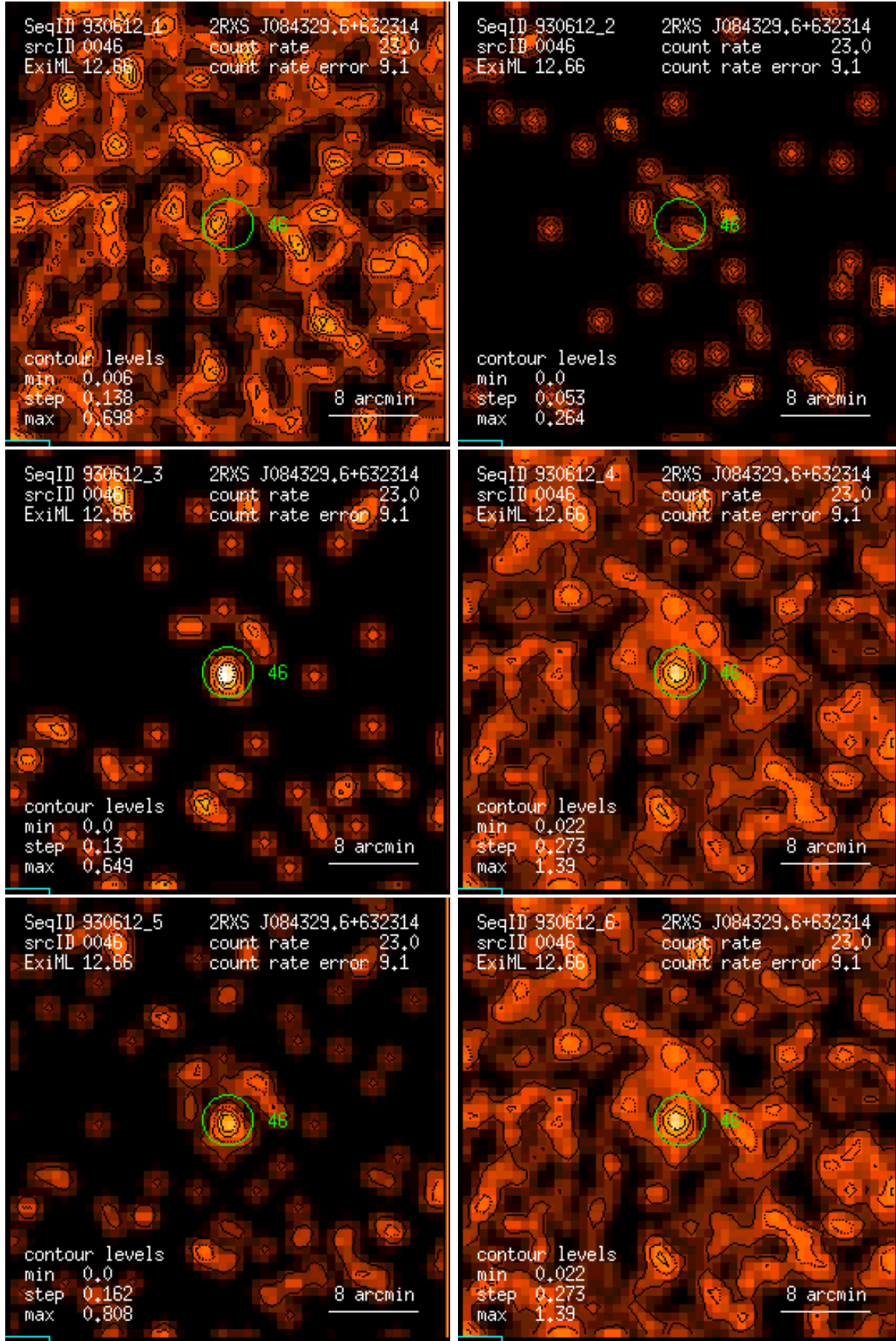
Figure 46: RASS 930612: detection 0046: band rate images, Gaussian filter: (1) PSPC channels 11 – 41, (2) 52 – 90, (3) 91 – 201, (4) 11 – 235, (5) 52 – 201, (6) 11 – 201. Broad band rates in counts/ks. Band rate contour levels in counts/ks/arcmin 2 .
