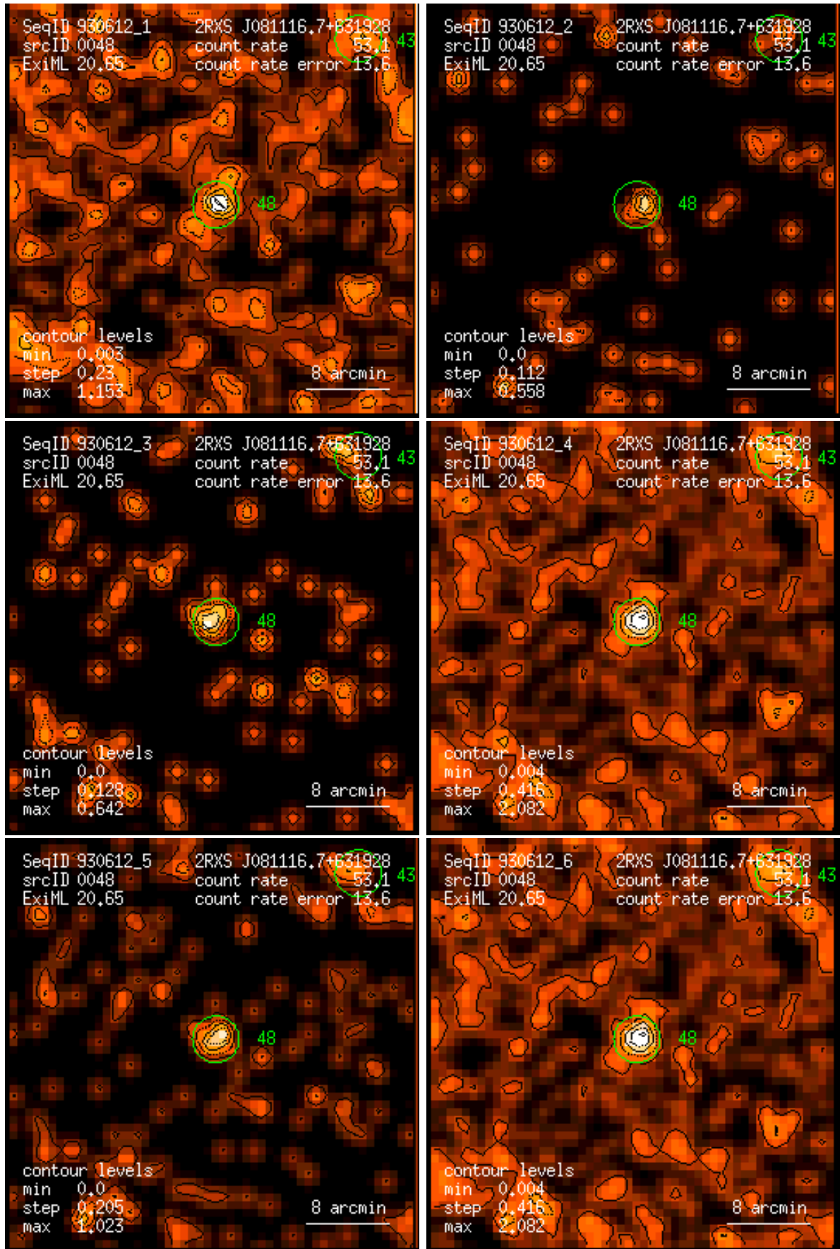
Figure 48: RASS 930612: detection 0048: band rate images, Gaussian filter: (1) PSPC channels 11 – 41, (2) 52 – 90, (3) 91 – 201, (4) 11 – 235, (5) 52 – 201, (6) 11 – 201. Broad band rates in counts/ks. Band rate contour levels in counts/ks/arcmin 2 .
