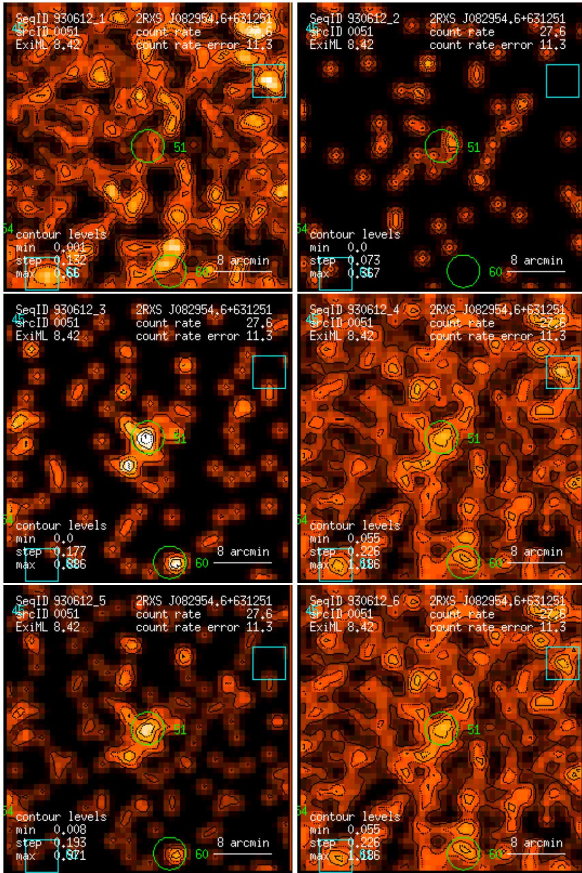
Figure 51: RASS 930612: detection 0051: band rate images, Gaussian filter: (1) PSPC channels 11 – 41, (2) 52 – 90, (3) 91 – 201, (4) 11 – 235, (5) 52 – 201, (6) 11 – 201. Broad band rates in counts/ks. Band rate contour levels in counts/ks/arcmin 2 .
